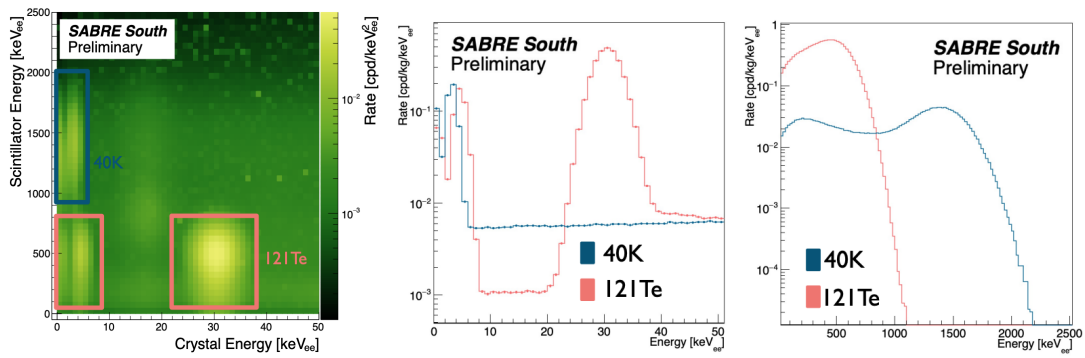
Figure 2: Left: energy depositions in both the crystal and liquid scintillator. Indicated in blue and pink are events due to ^{40}\text{K} and ^{121}\text{Te} . Centre: rate recorded in crystals from ^{40}\text{K} and ^{121}\text{Te} . Right: rate recorded in liquid scintillator from ^{40}\text{K} and ^{121}\text{Te} .
