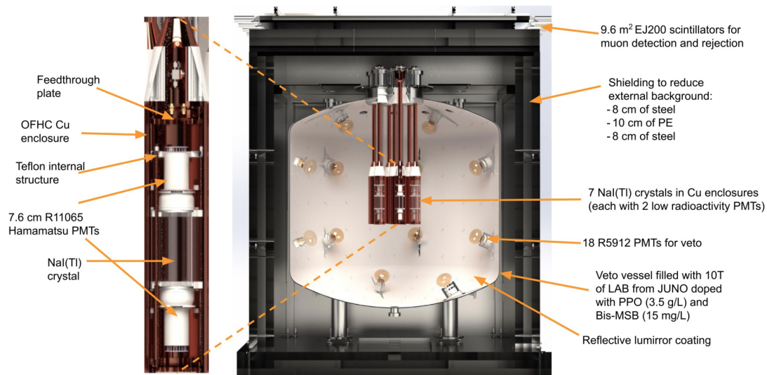
Figure 1: Rendering of the SABRE South detector.
