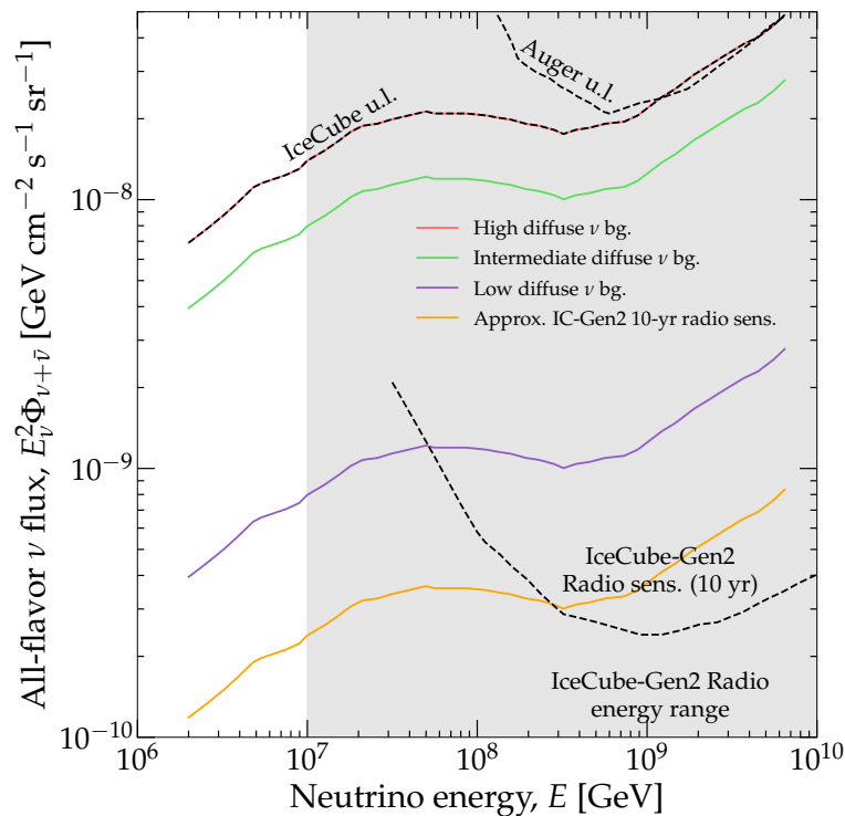
Figure 1: Benchmark diffuse UHE neutrino flux models used in our work. For comparison, we include the IceCube-Gen2 radio array sensitivity [5], and the upper limit from Auger [6].
