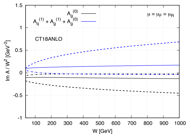
Figure 3: LO (black) and LO+NLO (blue) contributions to \text{Im } A/W^2 generated using CT18ANLO [3] global partons with \mu_F^2 = \mu_R^2 = Q_0^2, m_c^2 and 2m_c^2 (from bottom to top). \text{Im } A is the imaginary part of the amplitude.
