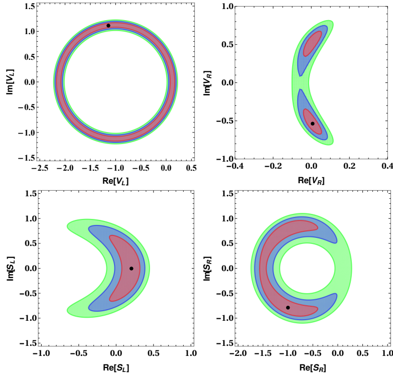
Figure 1: Constraints on various new coefficients obtained from \chi^2 fitting. Here red, blue and green colours represent the 1\sigma , 2\sigma and 3\sigma contours and the black dots represent the best-fit values.
