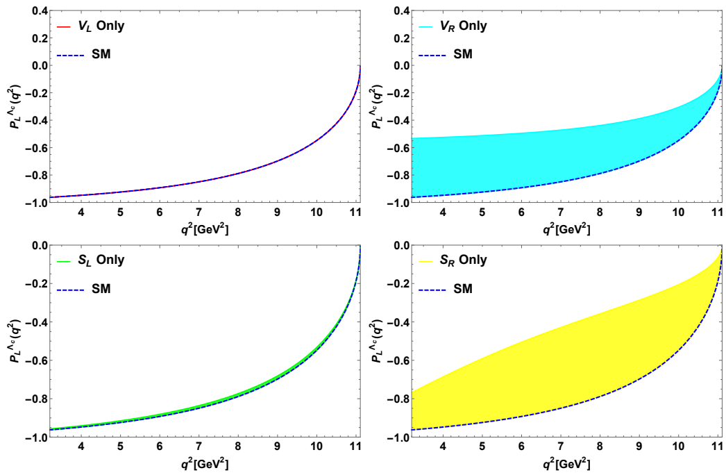
Figure 4: The q^2 variation of hadron polarization asymmetry of \Lambda_b \rightarrow \Lambda_c \tau \bar{\nu}_\tau process.
