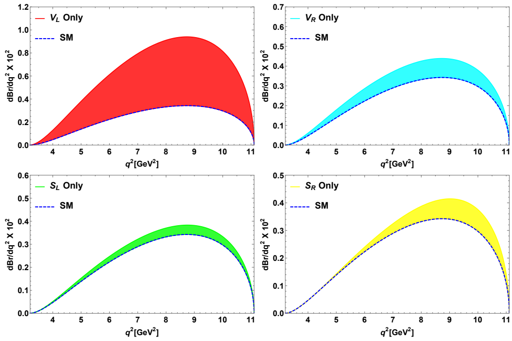
Figure 2: The q^2 variation of branching ratio of \Lambda_b \rightarrow \Lambda_c \tau \bar{\nu}_\tau process.
