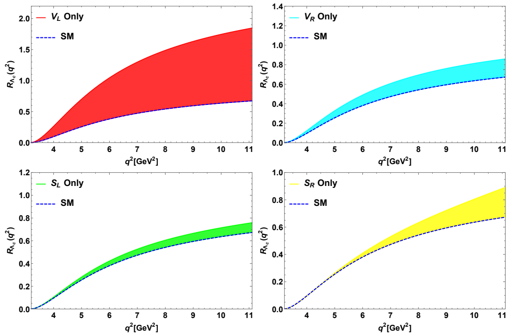
Figure 5: The q^2 variation of lepton non-universality of \Lambda_b \rightarrow \Lambda_c \tau \bar{\nu}_\tau process.
