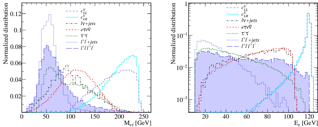
Figure 2: The two final state leptons invariant mass (left), and the energy of electron candidate (right) distributions are presented for c_{LR}^V = 0.1 and c_{LR}^V = 0.1 signal scenarios, at \sqrt{s} = 240 GeV [12].
