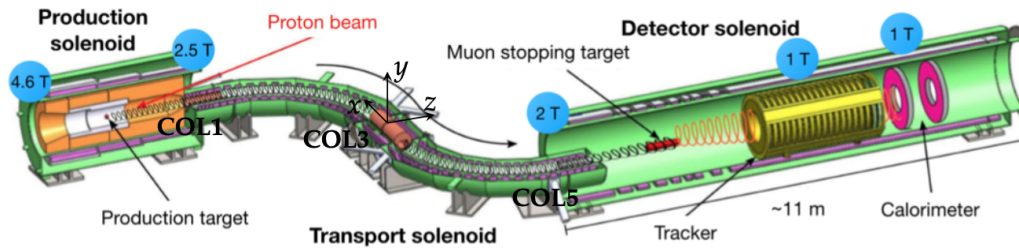
Figure 1: Schematic view of the Mu2e experiment [2].
