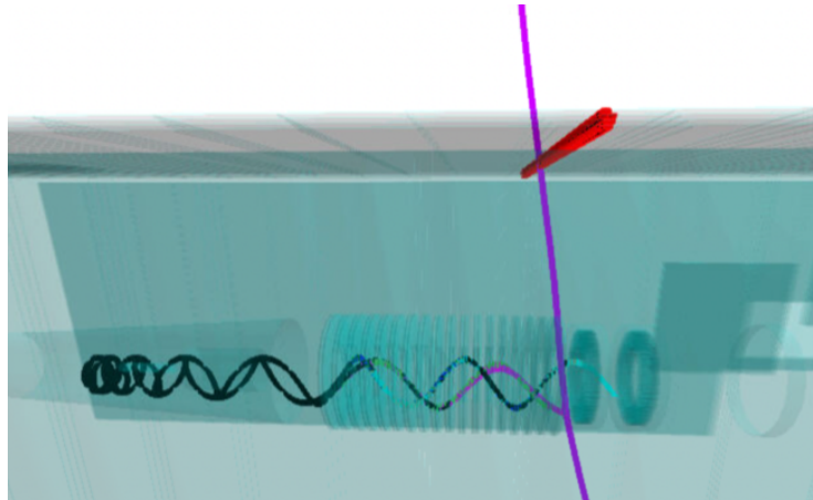
Figure 5: Event display of a multi-track event from cosmic ray interactions in the DS.
