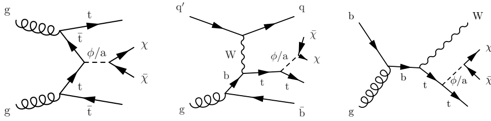
Figure 8: Diagrams for production of DM in association with a top quark pair or a single top quark: left, t\bar{t} +DM production; centre, t-channel t+DM production, and right, tW+DM production. Source: [16].
