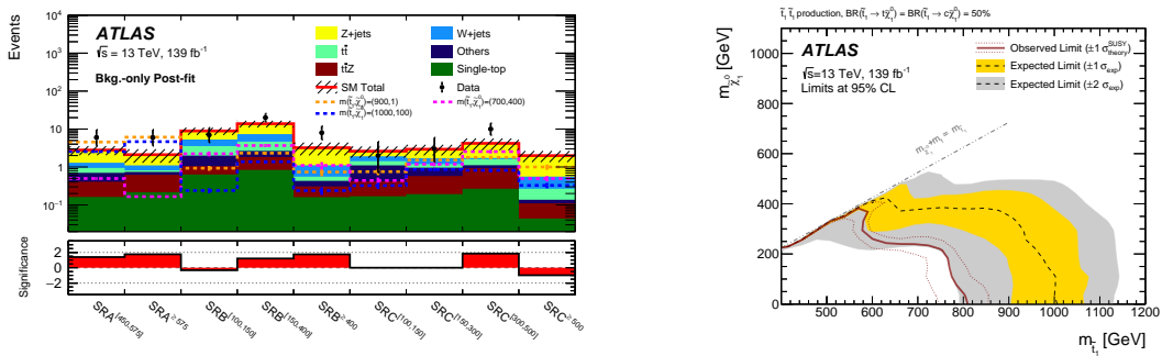
Figure 7: Left: Post-fit agreement with ATLAS data in the boosted and intermediate SRs for flavour violating stop quark production. Right: ATLAS limits on this model. Source: [15].
