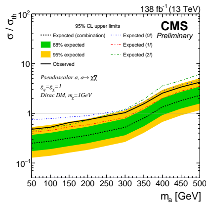
Figure 10: CMS limits on the combined cross section of t+\text{DM} and t\bar{t}+\text{DM} as a function of pseudoscalar mediator mass. Source: [16].
