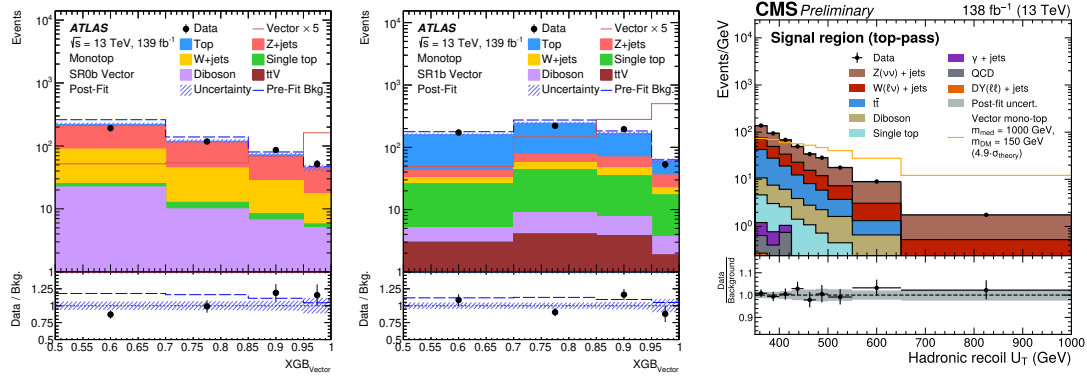
Figure 2: Signal regions for the ATLAS [5] 0b (left) and 1b (centre) categories, and for the CMS [8] signal-enriched top-pass category (right).
