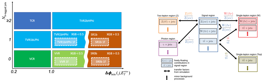
Figure 3: Left: the control, validation and signal regions for the ATLAS analysis (source: [5]). Right: the signal and control regions and transfer factors in the CMS analysis (source: [8]).
