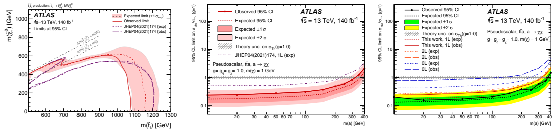
Figure 6: Comparisons of latest ATLAS 1l results [9] (red lines) with the previous re-sult published in [14] (purple lines) for stop quark pair production (left) and t\bar{t} + \text{DM} production via pseudoscalar mediator (center), and, right the combination of pseudoscalar t\bar{t} + \text{DM} limits with existing results in the 0 and 2 lepton channels.
