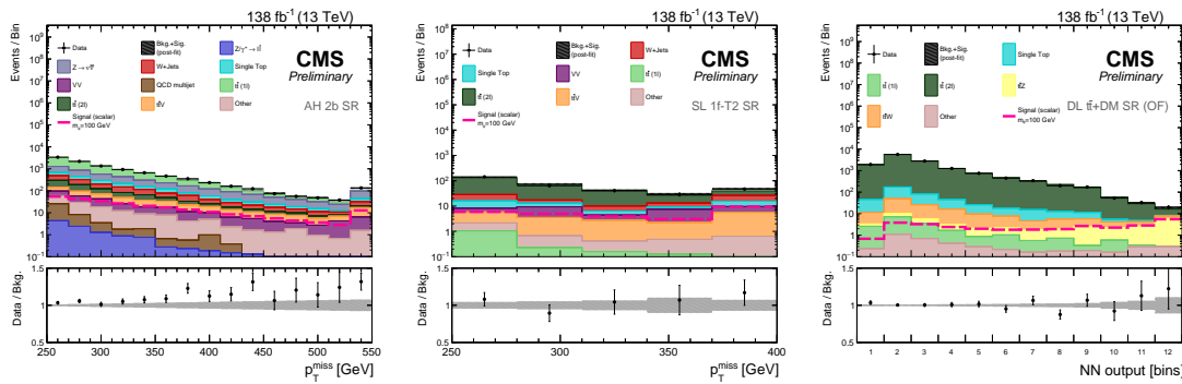
Figure 9: Example SRs for the combined CMS t+DM and t\bar{t} +DM search. Left, the 0 lepton, \geq 2 b jet SR; centre, the 1 lepton, 1 b jet, \geq 1 forward jet, high topness SR; right, the 2 lepton different flavour, \geq 2 b jet SR. Source: [16].
