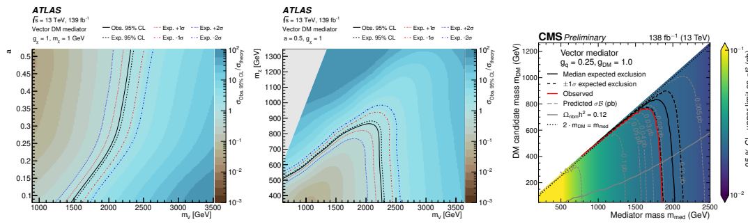
Figure 4: Left, the ATLAS limits on the mass of the mediator, m_V , and the coupling to the SM, a , for DM mass, m_\chi = 1 GeV; centre, the ATLAS limits on m_V and m_\chi for a = 0.5 (source: [5]). Right, the CMS limits on mediator mass, m_{\text{med}} , and DM mass, m_{\text{DM}} , for a coupling to the SM of 0.25 (source: [8]). All have a DM coupling of 1.0.
