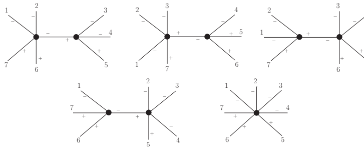
Figure 5: Contributions to the 7-point (----++) NNMHV amplitude. (Source of the figure: Ref. [8].)
