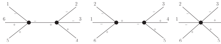
Figure 4: Contributions to the 6-point (---++) NMHV amplitude. (Source of the figure: Ref. [8].)
