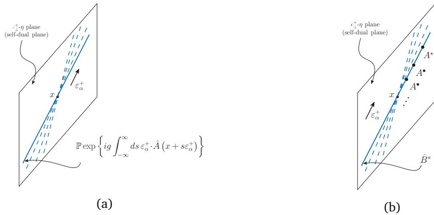
Figure 1: Left: The straight infinite Wilson line B^\bullet living on the self-dual plane spanned by \varepsilon_\alpha^+ = \varepsilon_\perp^+ - \alpha\eta and integrated over all \alpha (the dashed, tilted Wilson lines represent the change of \alpha ). Right: The B^* field can be seen as the straight infinite Wilson line similar to the one on the left, but here one A^\bullet field has been substituted by the A^* field in the expansion (with a suitable symmetry factor). (Source of the figure: Ref. [7].)
