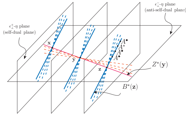
Figure 2: The geometric depiction of the Z^* field (the structure of Z^\bullet is fairly similar). Z^* field is a Wilson line (with exactly the same analytic form as B^\bullet ) of only B^* fields on anti-self-dual plane. Notice, each vertical plane is self-dual plane with B^* embedded in it as was shown in Fig. 1b. (Source of the figure: Ref. [8].)
