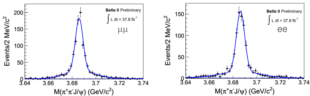
Figure 3: \psi(2S) state peaking in the J/\psi \pi^+ \pi^- invariant mass distribution for the ISR process e^+ e^- \rightarrow \pi^+ \pi^- J/\psi .
