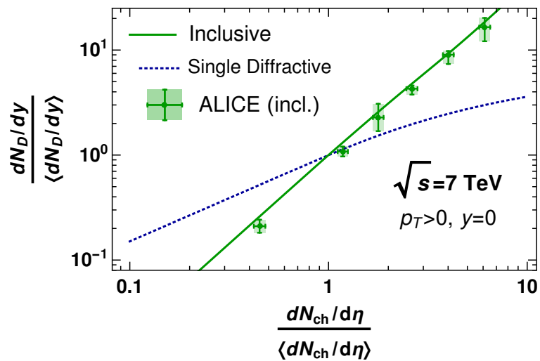
Figure 2: Results for the multiplicity dependence of inclusive and single diffractive production of D -mesons in LHC kinematics. For inclusive production we take into account both prompt and nonprompt mechanisms. The experimental data are for the multiplicity dependence of inclusive production from ALICE [1], and it is assumed that all particles are collected at central rapidities in rapidity window |y|, |\eta| \lesssim 1 .
