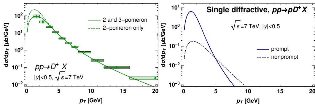
Figure 1: The D^+ -meson production cross-section as a function of transverse momentum p_T . Left and right plots correspond to inclusive and single diffractive production at central rapidities respectively. As explained in the text, the three-pomeron contribution in left-hand side is not positively defined due to interference diagrams, so its inclusion decreases the overall result. The experimental data are from [31–33].
