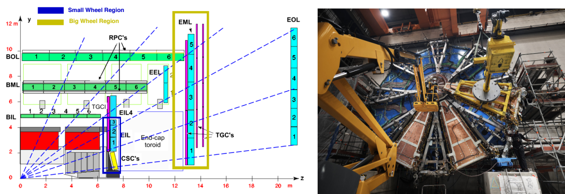
Figure 1: One of several detector systems in the ATLAS Muon Spectrometer (left), the New Small Wheel [3] is currently being assembled at CERN (right).
