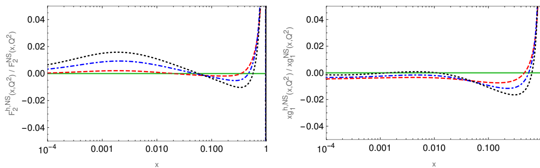
Figure 4: Left: The relative contribution of the heavy flavor contributions due to c and b quarks to the structure function F_2^{\text{NS}} at \text{N}^3\text{LO} ; dashed lines: 100 \text{ GeV}^2 ; dashed-dotted lines: 1000 \text{ GeV}^2 ; dotted lines: 10000 \text{ GeV}^2 . Right: The same for the structure function xg_1^{\text{NS}} at \text{N}^3\text{LO} . From [122].
