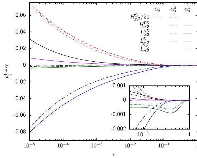
Figure 2: The different single mass heavy flavor contributions to the structure function F_2 at Q^2 = 100\text{GeV}^2 . From [120].
