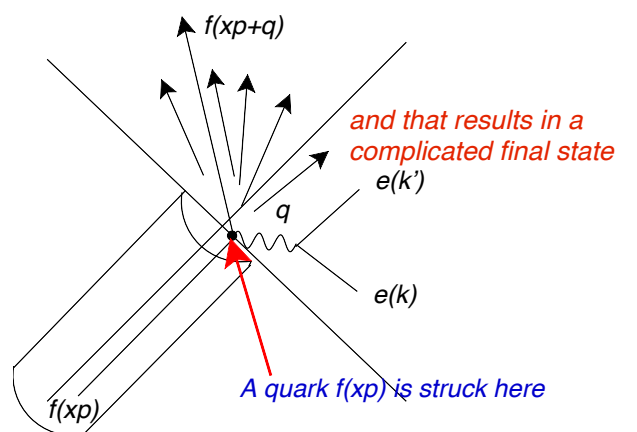
Figure 2: A typical event in deep-inelastic scattering.
