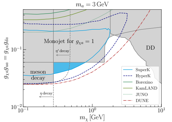
Figure 2: The constraints on the couplings including Borexino.
