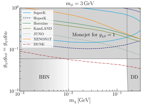
Figure 1: The constraints on the couplings with the mass scale in the form factor \Lambda_a = 1.03 \text{ GeV} .
