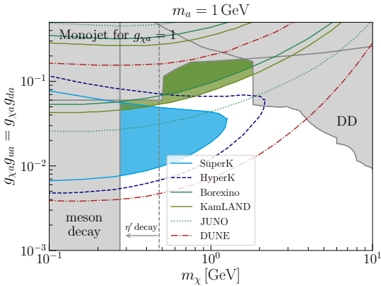
Figure 2: The constraints on the couplings including Borexino.
