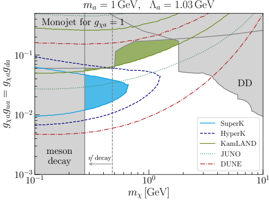
Figure 1: The constraints on the couplings with the mass scale in the form factor \Lambda_a = 1.03 \text{ GeV} .
