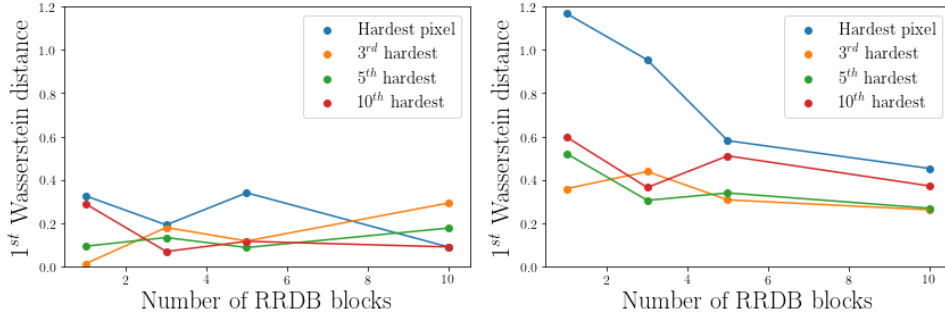
Figure 11: Dependence of the performance of super resolution networks on the number of internal RRDB blocks (See Fig. 2). Performance is measured via the one dimensional Wasserstein distance between the distribution of quantities over true high-resolution images and the super-resolution images. Quantities examined are the energy of the leading pixel, subleading, etc. Left (right) shows results for networks trained on top-quark (QCD) jets and applied to top-quark (QCD) jets.
