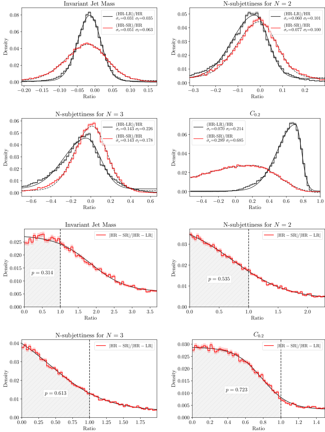
Figure 7: Distribution of the relative difference in a given high-level observable for per-jet top-jet triplets LR, SR, and HR. In the upper panels we show the normalized deviations, while in the lower panels we show ratios of deviations from the LR truth. The quoted value p gives the fraction of jet triples for which SR is closer to the HR truth than LR truth, so SR has added relevant information.
