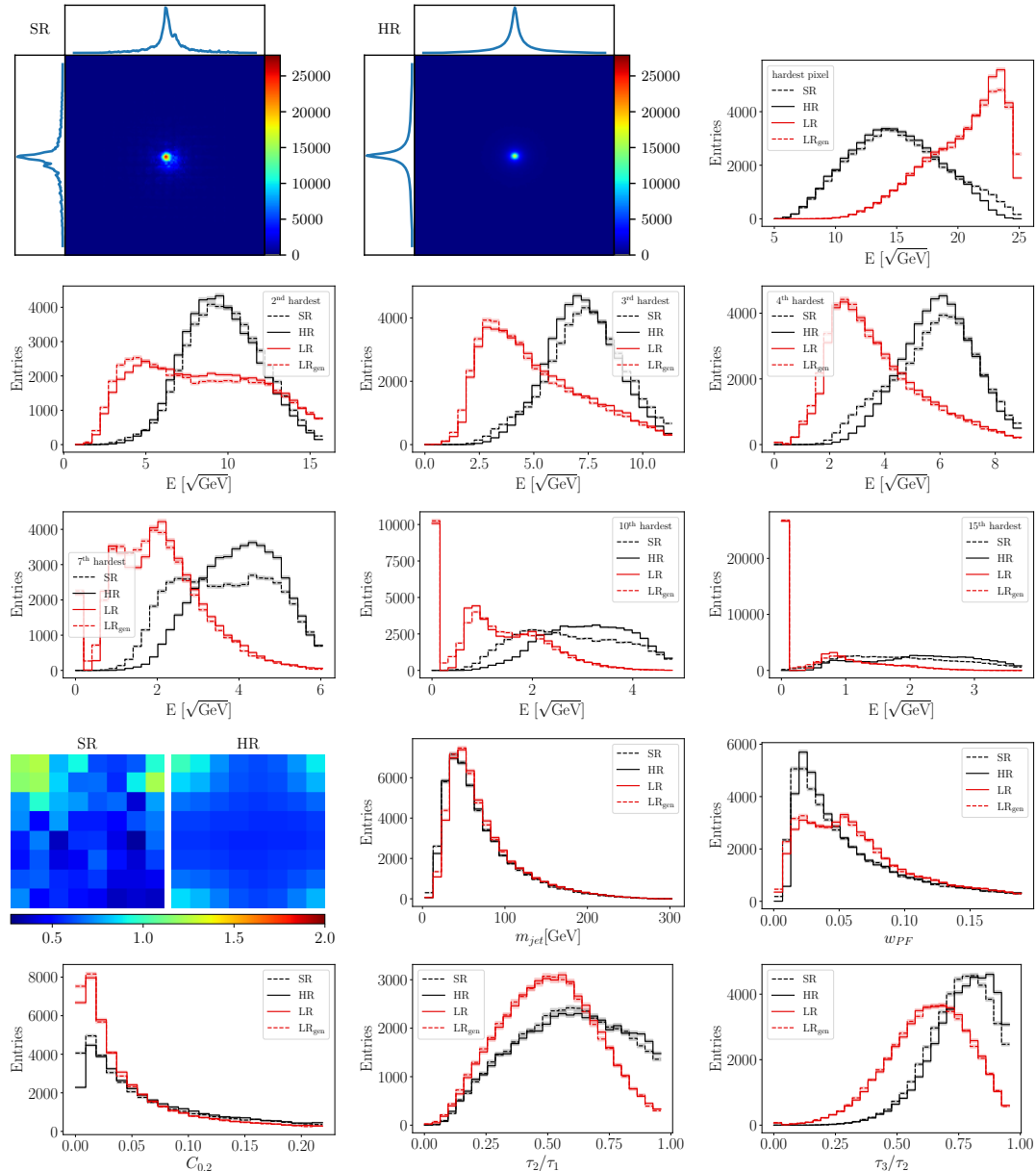
Figure 4: Demonstration of the performance of a network trained on QCD-jets and applied to QCD-jets. Top left are averages of the HR and SR images, followed by distributions of the square-root of the energy of leading pixels, sub-leading, etc. Also shown are average (f \times f) -patches for the SR and the HR images, and distributions of high-level jet observables, see text for definitions. The zero-bin in energy collects jets with too few entries.
