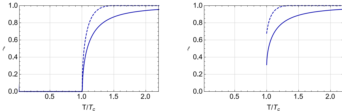
FIG. 4: SU(2) (left) and SU(3) (right) Polyakov loops as obtained using the self-consistent background field approach [19] (dashed) or the present center-symmetric background approach (plain).
