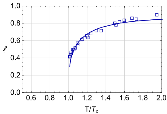
FIG. 5: Comparison of our SU(3) Polyakov to the lattice data of Refs. [49, 50].
