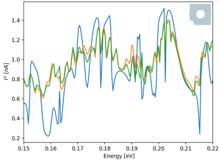
Figure 5: AC spin currents generated by the time-dependent Rashba SOI in the absence of a bias voltage are plotted as a function of the Fermi energy. In the high-frequency regime, the numerical Floquet results (green) are compared to the adiabatic approximation (blue) and the spin current in y -direction calculated from the time-dependent spin voltage, Eq. (48) (orange). The system size is L = 50a , and the Rashba SOI is \alpha_R(t) = k_{so} \sin(\Omega t) with k_{so}L = 0.01 and \Omega\tau \approx 1.5 .
