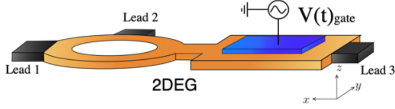
Figure 6: Setup of the dynamical spin-orbit based spin transistor with the top terminal (Lead 2) controlled electrostatically. The AC gate voltage in the right cavity induces a dynamical Rashba SOI, which creates an AC spin current that flows into the left cavity. There, due to a spatially inhomogeneous Rashba SOI, the spin current is transformed into a nonzero charge current in the multiterminal system. The charge current vanishes in the two-terminal system.
