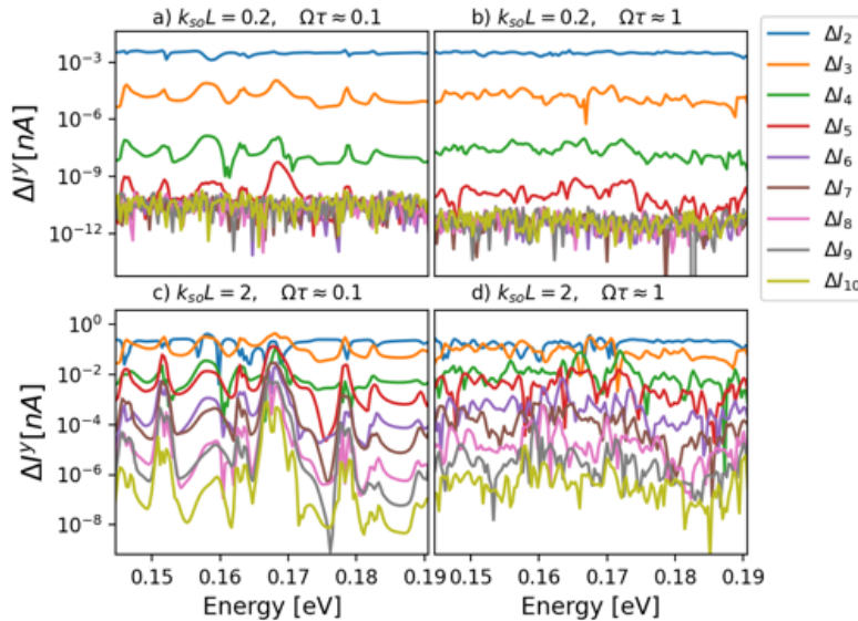
Figure 10: The convergence in n of the AC spin currents generated by the time-dependent Rashba SOI, where \Delta I_n = (I_n - I_{n-1})/I_n and I_n is the current calculated with maximum Floquet states N . The parameters correspond to \Omega\tau \approx 0.1 and 1, and k_{so}L = 0.2 and 2.
