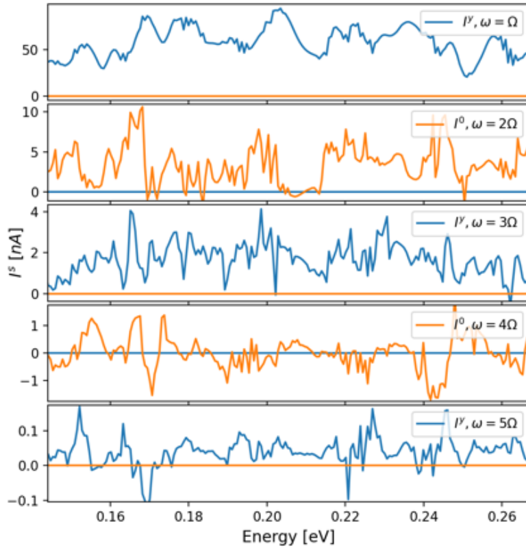
Figure 11: High harmonic generation of AC spin currents in y direction (blue) and AC charge current (orange) in the presence of the time dependent Rashba SOI. The currents are plotted as a function of the Fermi energy where Rashba SOI \alpha(t) = k_{so} \sin(\Omega t) , k_{so}L = 1 , L is the system size in x direction and \Omega\tau \approx 1 .
