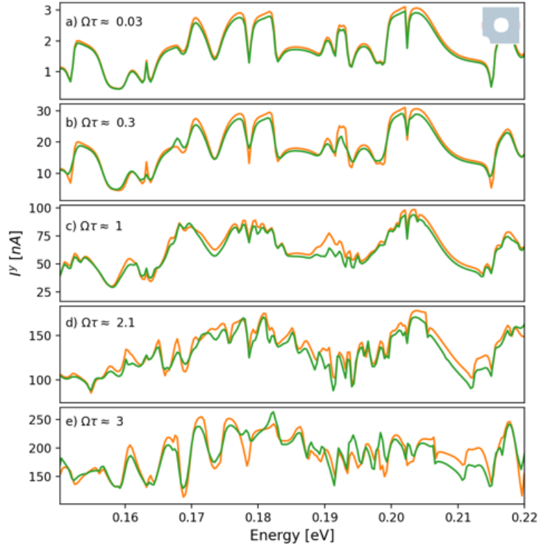
Figure 4: AC spin currents generated by the time-dependent Rashba SOI in the absence of any charge bias are plotted as a function of the Fermi energy. The numerical Floquet results (green) are compared to the spin current in y direction in the presence of the time-dependent spin voltage (orange). The spin currents (orange) are calculated using Eq. (42) in the low-frequency regime in panels a) and b) and by Eq. (48) in the high-frequency regime in panels c), d) and e). The system size is L = 50a and the Rashba SOI is \alpha_R(t) = k_{so} \sin(\Omega t) with k_{so}L = 1 . The frequency values are indicated at the top left corner of each panel, \Omega\tau \approx 0.03, 0.3, 1, 2.1 and 3 in panels a) and b), etc., respectively. The system geometry is shown in the top right inset.
