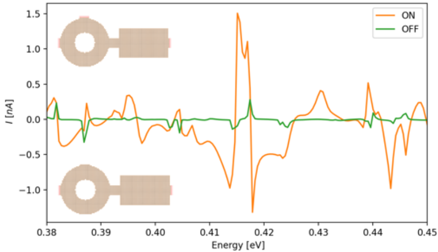
Figure 8: Comparison On/Off state of the Dynamical spin transistor. AC charge currents in Lead 1, see Fig. 6, as a function of the Fermi energy is generated by the time-dependent and spatially inhomogeneous Rashba SOI. Numerical results based on the Floquet formalism are calculated for both the presence and absence of the time-reversal symmetry. ... .... The dynamical Rashba SOI in the right half system is \alpha_R(t) = k_{so} \sin(\Omega t) with k_{so}L = 1 and the spatially inhomogeneous Rashba SOI in the left half system (the ring) is \alpha_R(\mathbf{x}) = k_{so}(L - y)/L . The size of each system part is L = 50a and the driving frequency is \Omega\tau \approx 0.1 .
