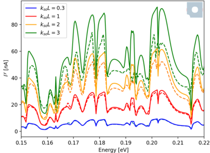
Figure 3: Comparison of the AC spin currents generated by the spin-dependent voltage (Eq. (42), solid line) and numerically (dashed) directly for the time-dependent Rashba SOI \alpha_R(t) = k_{so} \sin(\Omega t) with \Omega\tau \approx 0.3 and varying values k_{so}L = 0.3 (blue), 1 (red), 2 (orange), 3 (green). The AC spin currents are plotted as a function of the Fermi energy.
