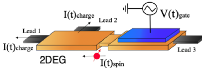
Figure 1: Sketch of the dynamical spin transistor. The on/off state of the spin transistor can be controlled by opening the top terminal (Lead 2). A time-dependent top gate voltage generates a spin current on the right. This is read out as a nonzero charge current on the left part in the multiterminal system via spatially inhomogeneous Rashba coupling. In the two-terminal system the charge current vanishes.
