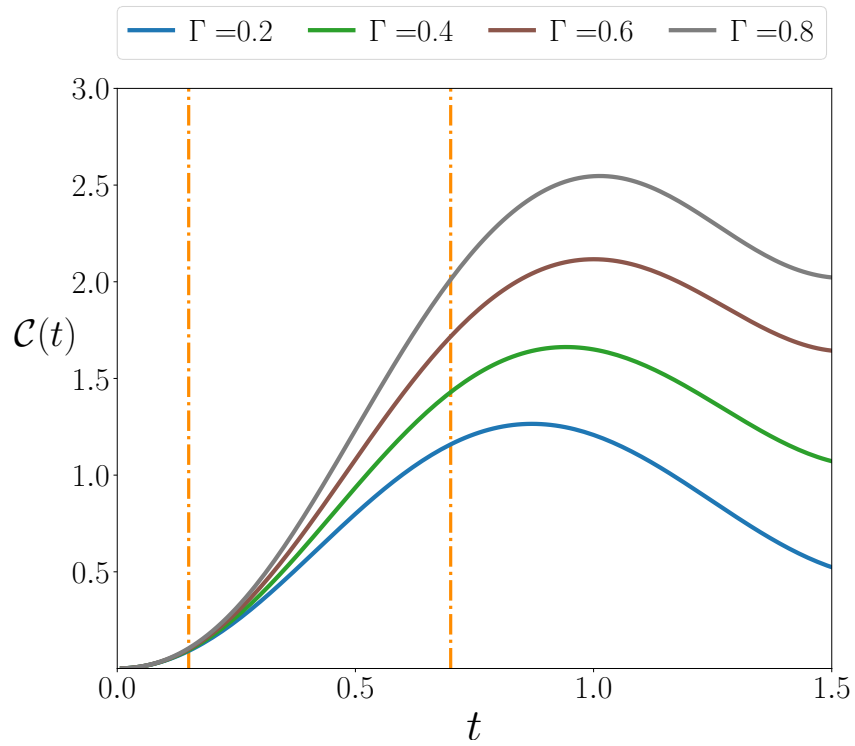
FIG. 3: The time development of the commutator squared value is shown for different rates ( \Gamma ) of the smooth quench. The dashed-dotted lines represent the points in the plot with increasing ramps which we use to extract the Lyapunov exponent
