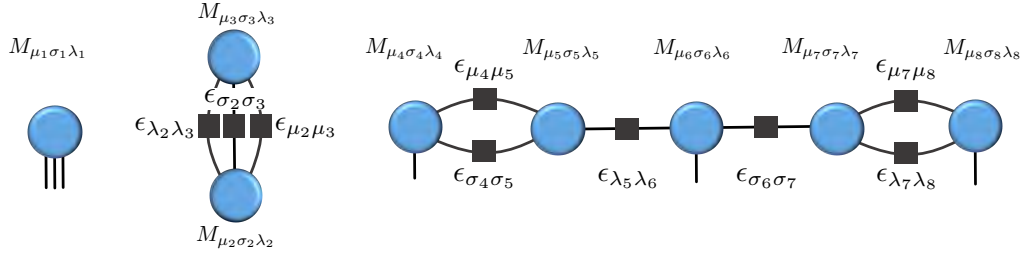
FIG. 17. MPS diagrammatic representation of DNA for N = 8 . We have identified M_{I_1^{(1)} I_1^{(2)} I_1^{(3)}}^{I_1} = M_{\mu_1 \sigma_1 \lambda_1} . Here, the diagram is for f_{N_L, \nu}^{\{\lambda\} \text{ broot}} = (z_1 \bar{z}_1)^{\mu_1 + \sigma_1 + \lambda_1} (z_4 \bar{z}_4)^{\lambda_4} (z_6 \bar{z}_6)^{\mu_6} (z_8 \bar{z}_8)^{\sigma_8} \times D_{\alpha_1 \alpha_2}^3(2, 3) D_{\alpha_1 \alpha_2}^2(4, 5) D_{\alpha_1 \alpha_2}(5, 6) D_{\alpha_1 \alpha_2}(6, 7) D_{\alpha_1 \alpha_2}^2(7, 8) where \mu_1 = \sigma_1 = \lambda_1 = \lambda_4 = \mu_6 = \sigma_8 = 1 . The number of bonds can easily be read from the graph: \mathbf{b}_i = (0, 3, 0, 2, 1, 1, 2) .
