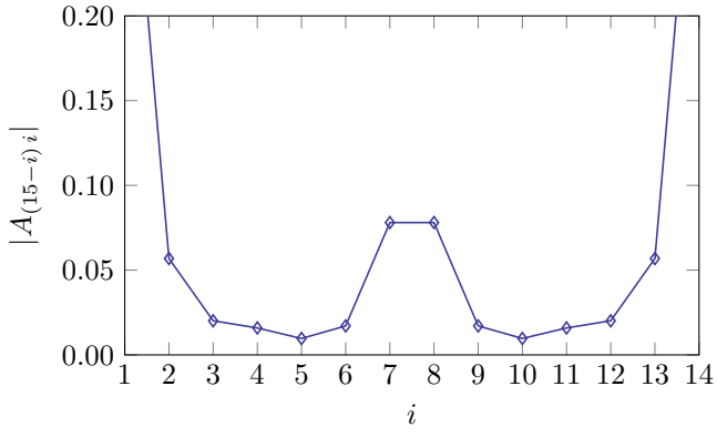
Absolute values of the anti-diagonal elements of the matrices A and B as shown in the lower panels (parity sector containing the |\mathbb{Z}_2\rangle state) of Fig. 3 in the manuscript. We label rows and columns by indices 1, 2, \dots, 14 .
