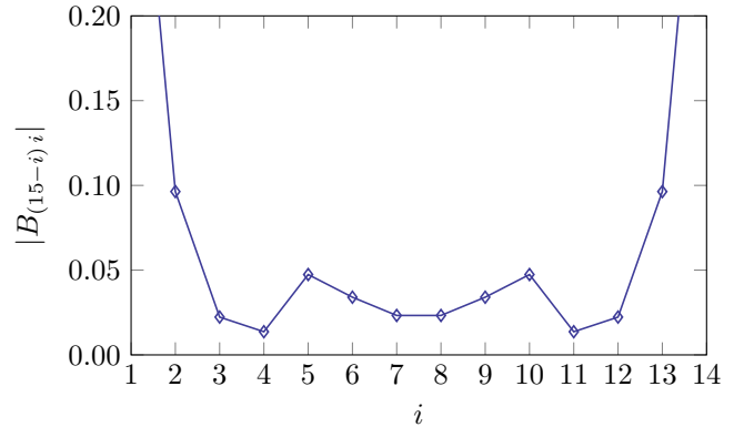
Absolute values of the anti-diagonal elements of the matrices A and B as shown in the lower panels (parity sector containing the |\mathbb{Z}_2\rangle state) of Fig. 3 in the manuscript. We label rows and columns by indices 1, 2, \dots, 14 .
