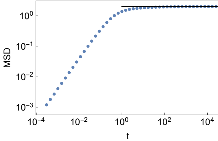
Figure 3: Mean-squared displacement of harmonic chain driven by center-of-mass conserving noise. Markers denote exact results. Solid lines represent long time asymptotic behavior: \text{MSD} \sim 2 \langle u_1^2 \rangle . For simplicity, we set K = 1 and T = 1 .
