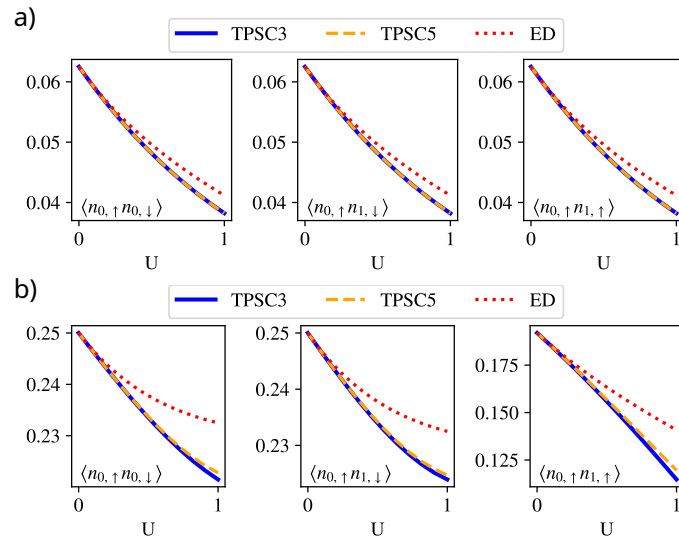
Figure 7: Comparison between TPSC and ED at \beta = 2 , for different U at J = 0 at quarter filling (panel a) and J -combinations with a kinetic inter-orbital coupling of unit strength (panel b). For these comparisons we include the zeroth order self-energy correction.
