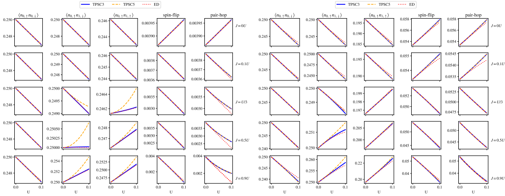
Figure 6: Comparison between TPSC TPSC3 (blue), TPSC5 (yellow) and ED (red) for the model defined in Eq. (144) at \beta = 2 on the left and \beta = 0.5 on the right, for different U at J = 0 at quarter filling (panel a) and with an inter-orbital coupling of unit strength (panel b) J combinations. For these comparisons we include the zeroth order self-energy correction in both TPSC variants.
