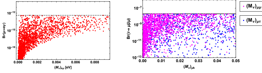
Figure 4: Left plot shows the correlation between the BR of \mu \rightarrow e\gamma with respect to m_{e\mu} and right one shows BR for \tau \rightarrow \mu\bar{\mu}\mu with the mass element m_{\mu\mu} and m_{\mu\tau} .
