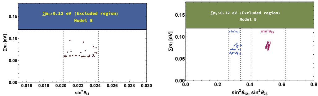
Figure 1: Left (right) plot shows the variation of \sum_i m_i with \sin^2 \theta_{13} ( \sin^2 \theta_{12} , \sin^2 \theta_{23} )
