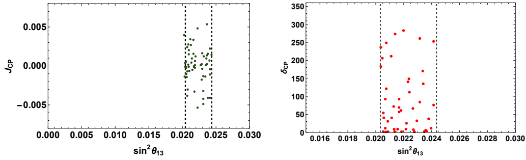
Figure 3: Left (right) plot shows the variation of J_{CP} ( \delta_{CP} ) with \sin^2\theta_{13}
