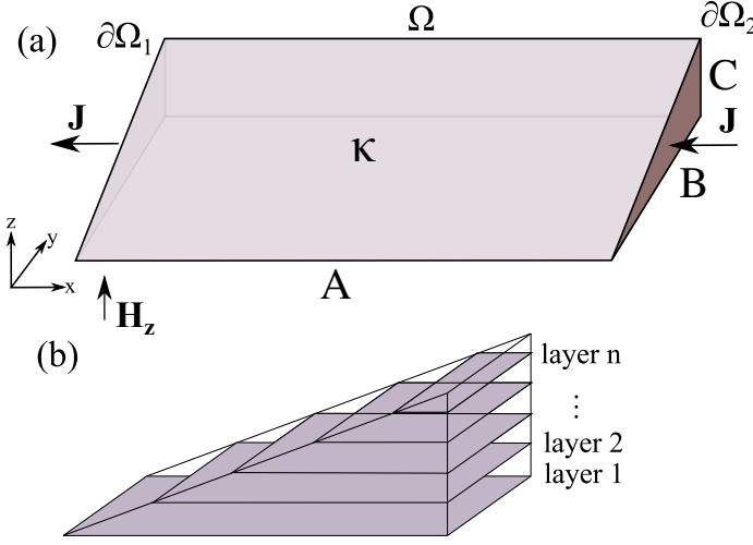
FIG. 1. (a) Schematic representation of the superconducting meso-wedge geometry. The dimensions of the external numerical mesh are A = 30\xi , B=C = 15\xi . (b) Real three-dimensional superconducting sample with meso-wedge geometry and its projection of n -layers for the superconducting meso-wedge sample. The inclusion of external/transport currents ( \mathbf{J} ) in -\hat{x} -direction- is given by the lateral faces \partial\Omega_i , i = 1, 2 , the external magnetic field ( \mathbf{H} = \mathbf{H}_z ) is in the \hat{z} -direction.
