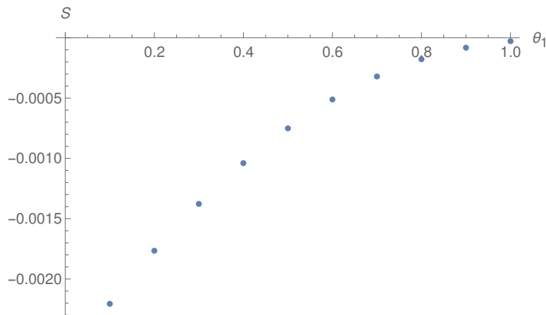
Figure 2. The plot of the six point function S in the short time limit \theta_2 \rightarrow \theta_1 . In this figure we have chosen arguments \theta_3 = \theta_4 = \pi , and \theta_5 = \theta_6 = 5\pi/3 .
