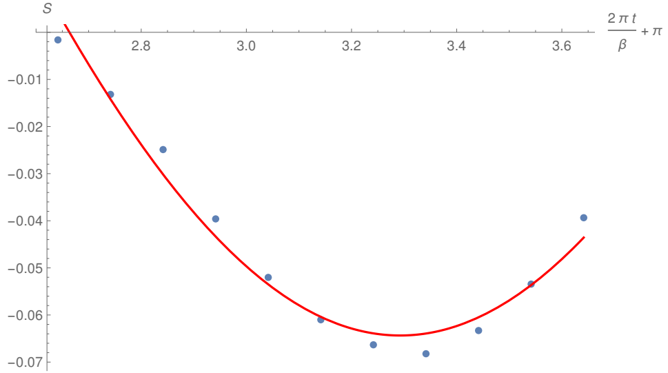
Figure 3. Plot of six-point OTOC computed numerically, for step-size = 0.08. The x-axis is given by \pi + 2\pi t/\beta . Dotted line are the data points while solid line is the fitted curve.
