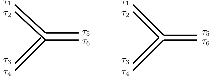
Figure 1. Contact (left) and Planar (right) diagrams for six point function. The double lines are dressed four point functions which include melonic corrections.
