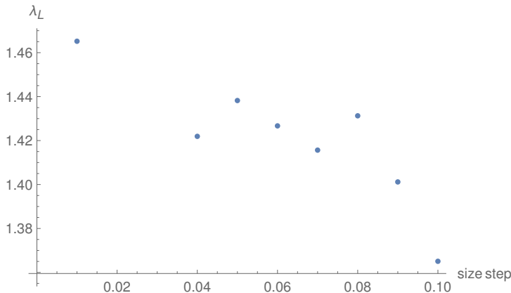
Figure 4. \lambda_L as a function of the step-size (from 0.01 to 0.1)
