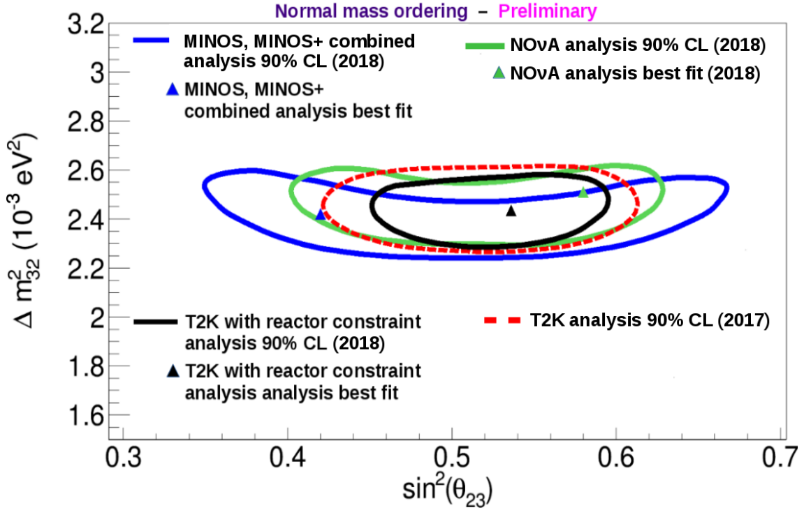
Figure 20: 90% confidence level 2D contours and best fit points for the \Delta m_{32}^2 and \theta_{23} for the T2K (dashed red), the T2K with reactor constraints (black), the NO \nu A experiment and the MINOS and MINOS+ experiments.
