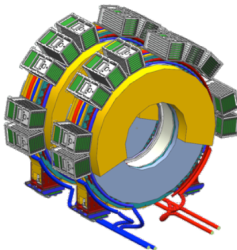
Figure 7: CAD drawing of the electromagnetic calorimeter. The crystals are located inside the aluminum rings, and the digitizing electronics are in the crates on the outside of the disks. The light blue area representing the support for the SiPMs and front end electronics, and the yellow area representing the envelope of the cables from the FEE to the digitizing electronics.
