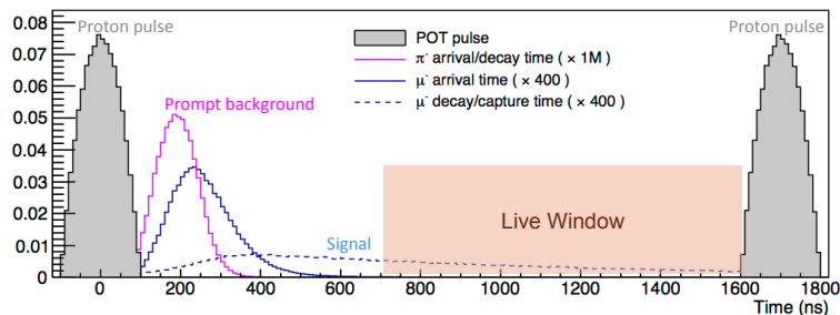
Figure 2: The Mu2e muon beam structure and live window compared to expected time distributions of backgrounds and signals.
