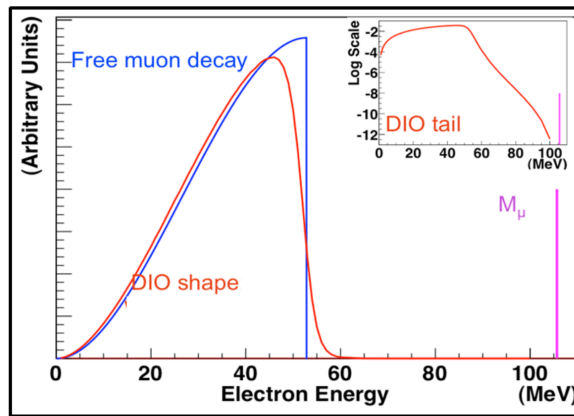
Figure 1: Energy spectrum of electrons produced by muon decay-in-orbit (red) compared with those from free muon decay (blue). Near the conversion endpoint at 105 MeV the decay-in-orbit spectrum falls as (E - E_{\text{endpoint}})^5 .
