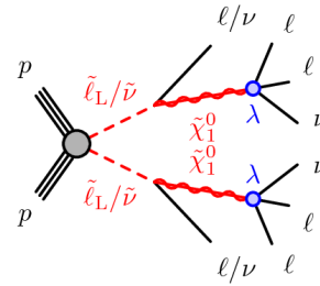
Figure 19: \tilde{l}_L/\tilde{\nu} NLSP [21].
