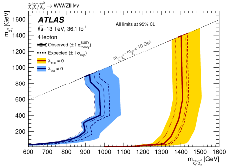
Figure 23: RPV wino W/Z NLSP [21].
