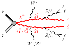
Figure 21: \tilde{\chi}_1^\mp \tilde{\chi}_1^\pm/\tilde{\chi}_2^0 [21].
