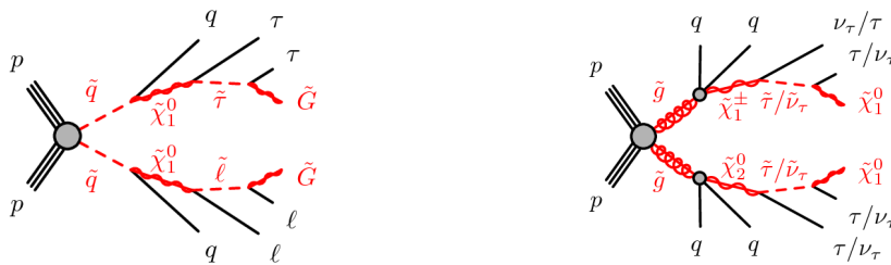
Figure 1: Diagrams illustrating example processes of the GMSB model (left), the scalar lepton \tilde{l} is preferentially a \tilde{\tau}_1 for high values of \tan\beta , and the simplified model (right) [4].
