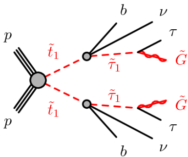
Figure 4: The simplified model for production and decay of SUSY particles considered [11].
