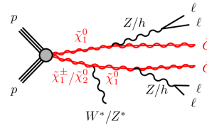
Figure 22: \tilde{\chi}_1^0 \tilde{\chi}_1^\pm/\tilde{\chi}_2^0 [21].
