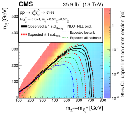
Figure 7: Exclusion limits at 95% CL for chargino-neutralino production with decays through \tilde{\tau} to final states with \tau leptons [15]. Figure 8: Exclusion limits at 95% CL for chargino pair production with decays through \tilde{\tau} to final states with \tau leptons [15].
