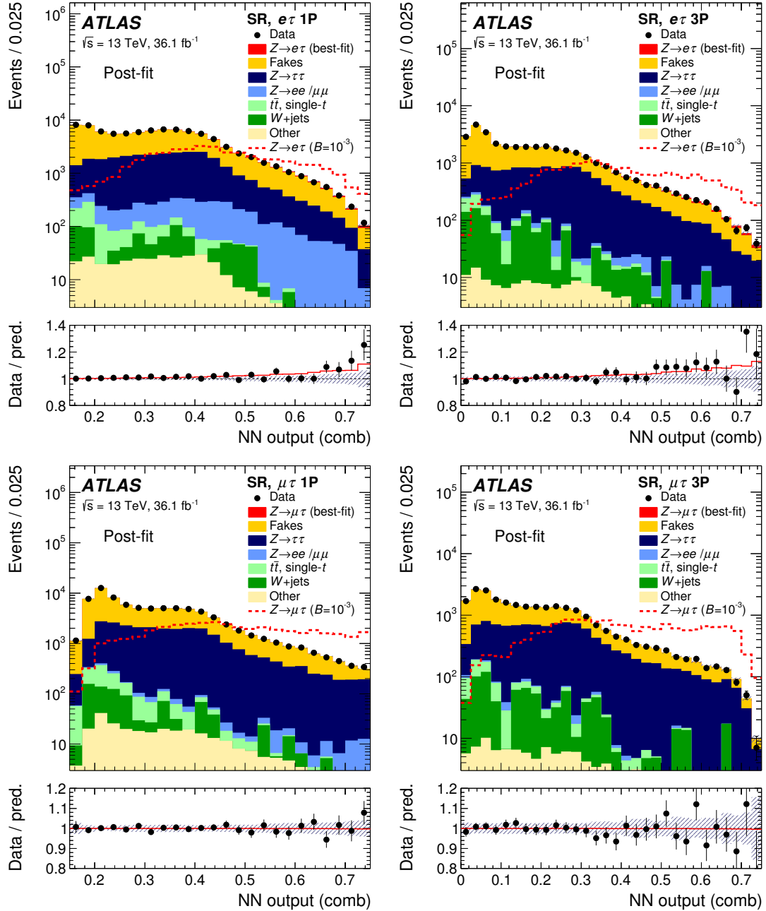
Figure 5: The distribution of the Neural Network classifier score for the Z \rightarrow e\tau (top) and Z \rightarrow \mu\tau (bottom) searches divided between the 1p and 3p decays respectively [17]. The lower panels quantify the agreement between background model and data. For the Z \rightarrow e\tau , the signal fixed to the best-fit branching ratio plus background is represented on this plot as a red line.
