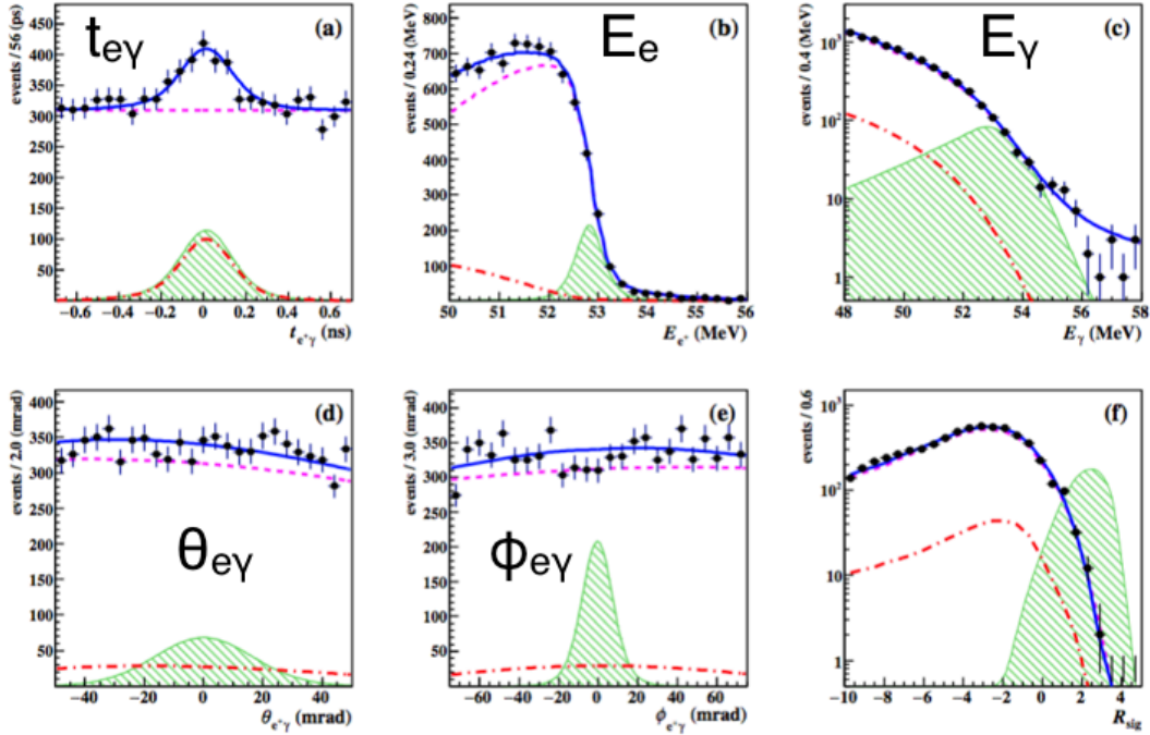
Figure 2: The best functions of each variable projected from the likelihood results for the full dataset, and the relative signal likelihood, R_{sig} with full data points. The blue solid line is the total fit result, the magenta dash line is the number of accidental backgrounds, and the red dot-dash line is the number of RMD.
