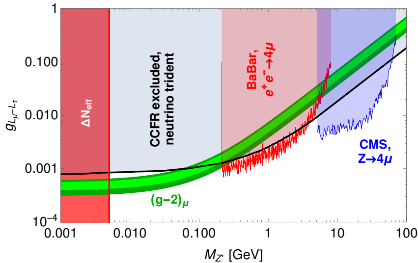
Figure 5: Constraints on U(1)_{L_\mu-L_\tau} without any Z-Z' mixing. Shown are the preferred region to resolve the muon's (g-2) at 1 and 2\sigma in green and exclusions from \Delta N_{\text{eff}} [57,58], BaBar [75], CMS [100], and neutrino trident production in CCFR [73,74].
