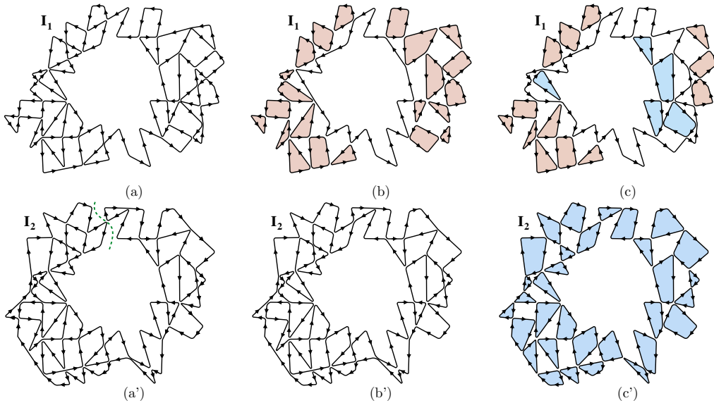
Figure 9: Interface graph \mathbf{I}_1 (top) and \mathbf{I}_2 (bottom). (a) and (a') are Eulerian circuits that wind and do not wind respectively around the central face. (b') decomposition of \mathbf{I}_2 into a clockwise and a counter clockwise circuits. (b) and (c) are examples of non-minimal Veblen decompositions" of \mathbf{I}_1 . (c') is the minimal Veblen decomposition of \mathbf{I}_2 .
