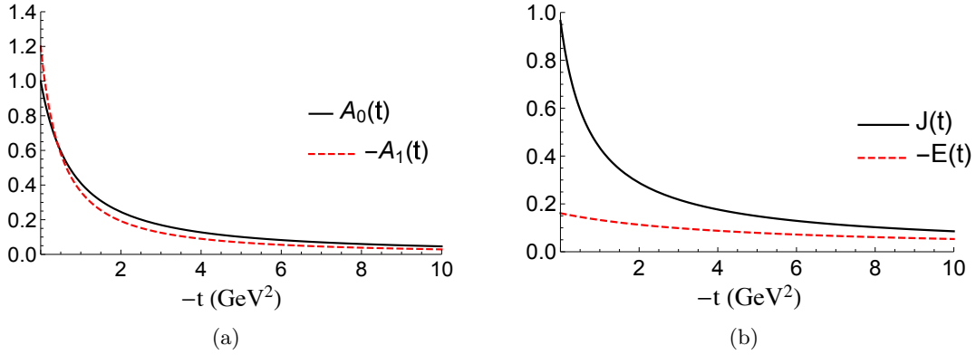
Figure 4: Some GFFs of the \rho meson. (a) A_0(t) and A_1(t) , and (b) J(t) and E(t) .
