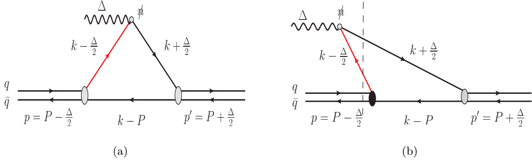
Figure 1: GPDs of the \rho meson. (a) Direct Feynman diagram contributed to the GPDs by the stuck quark ( q ) in the valence region, and (b) the stuck u quark in the non-valence region.
