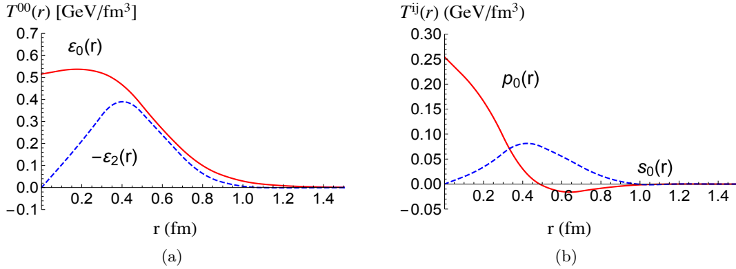
Figure 5: \rho meson mechanical properties. (a) mass distributions \epsilon_0(r) and \epsilon_2(r) , and (b) share force s_0(r) and pressure p_0(r) .
