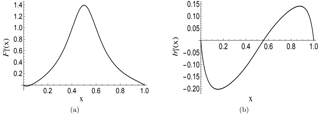
Figure 3: \rho meson structure functions. (a) F_1^u , and (b) b_1^u(x) contributed by the u quark, respectively.
