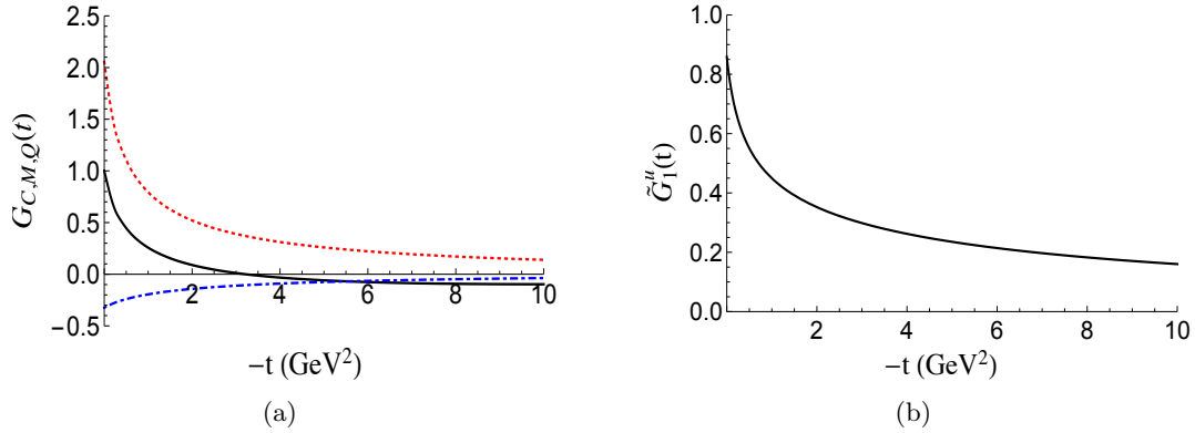
Figure 2: \rho meson form factors. (a) EM form factors, charge G_c (solid black curve), magnetic G_M (dashed red curve), and quadrupole G_Q (dotted-dashed blue curve) form factors, and (b) EW axial form factor \tilde{G}_1^u(t) contributed by the u quark.
