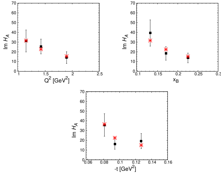
Figure 2: Imaginary part of CFFs given by Eq. (1) obtained from our model for H_q^{4\text{He}} . Our results (red stars) compared with data (black squares) [7]. From left to right, the quantity is shown in the experimental Q^2 , x_B and t = \Delta^2 bins, respectively. Analogous results for the real part of CFFs given by Eq. (2) are presented in [24].
