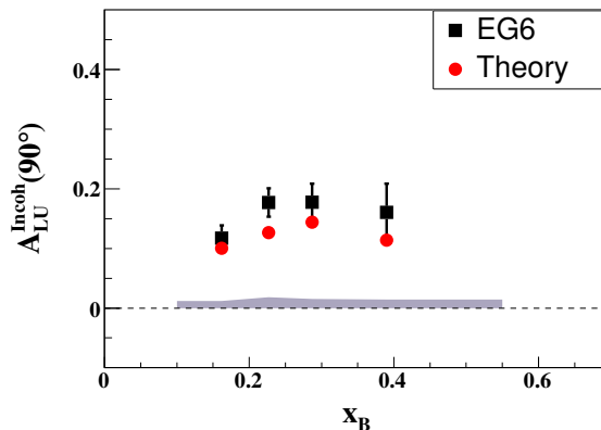
Figure 5: Azimuthal beam-spin asymmetry for the proton in {}^4\text{He} , A_{LU}^{Incoh} , Eq.(10), for \phi = 90^\circ : results of this approach [27](red dots) compared with data (black squares) [8]
