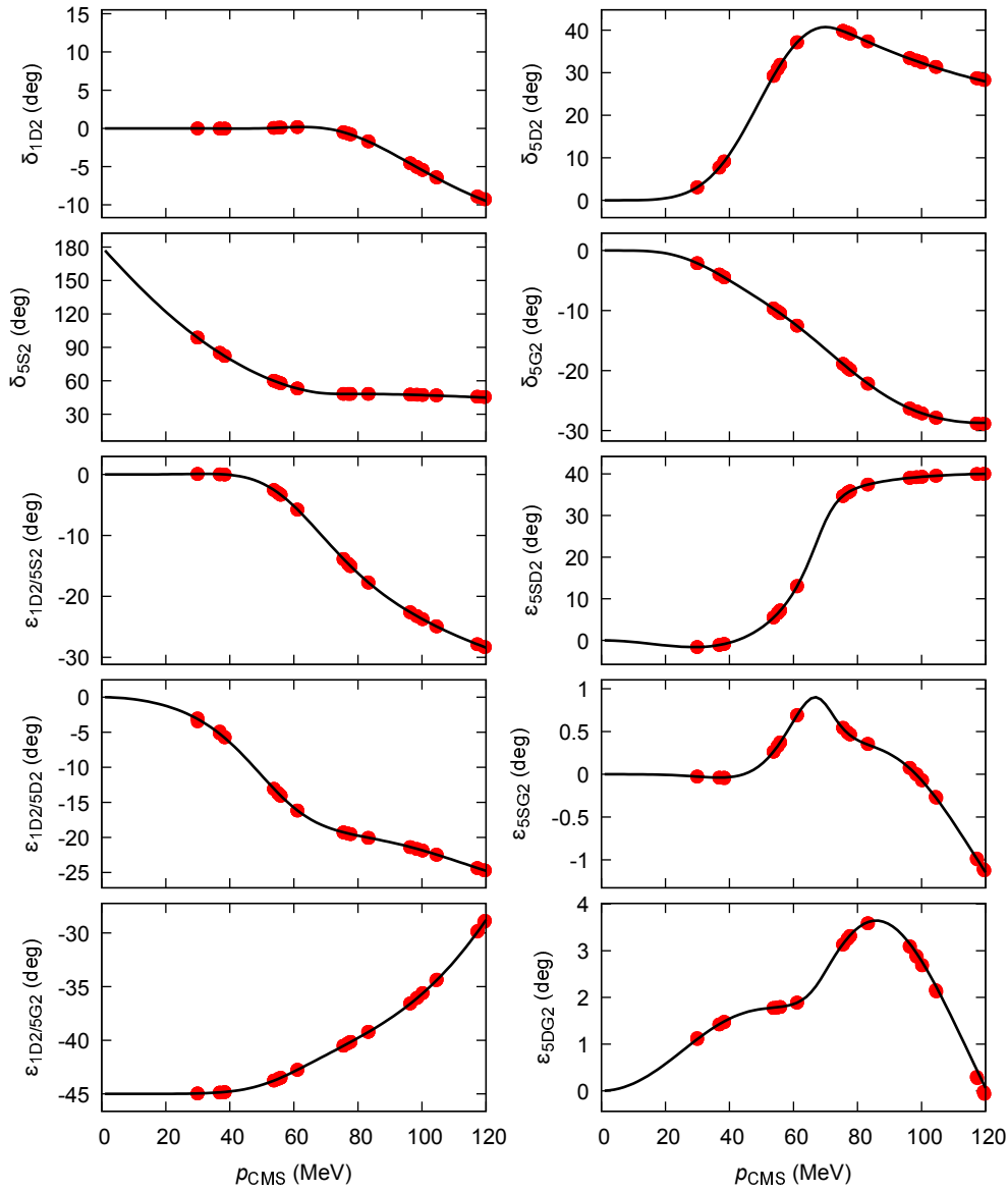
Figure 1: Phase shifts and mixing angles for the ^1D_2/{}^5SDG_2 -wave (black solid line: continuum; red points: lattice).
