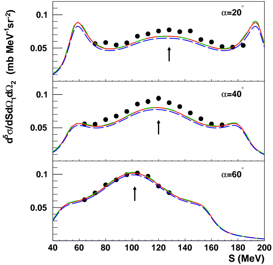
Figure 1: Deuteron breakup cross-section ( d(160 \text{ MeV})+p \rightarrow p+p+n ) for 3 different values of \alpha . Cross-section distributions are plotted against the value of the arc length along the kinematics ( S ) with the starting point ( S = 0 ) chosen arbitrarily at the point where E_2 reaches minimum (see Fig. 2). The central value corresponds to the star configuration (arrow). The theoretical predictions are plotted as lines (red solid: CD-Bonn+ \Delta +Coulomb, green chain: CD-Bonn+ \Delta , blue dashed: CD-Bonn+Coulomb) [5,15]. The normalisation of the experimental data is not finalised and does not contain e.g. effects due to with double-hits.
