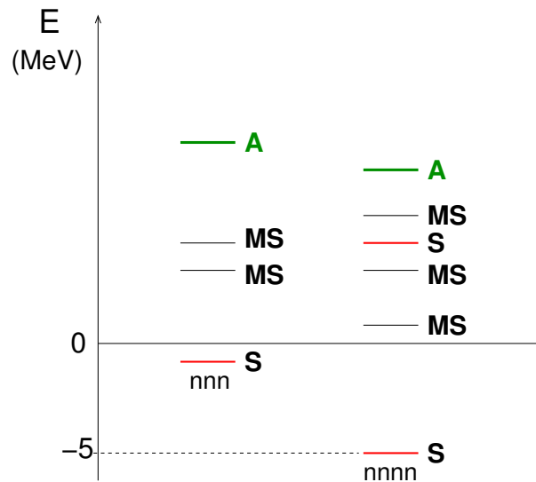
Figure 3: Schematic low level ordering of 3n and 4n in OH basis
