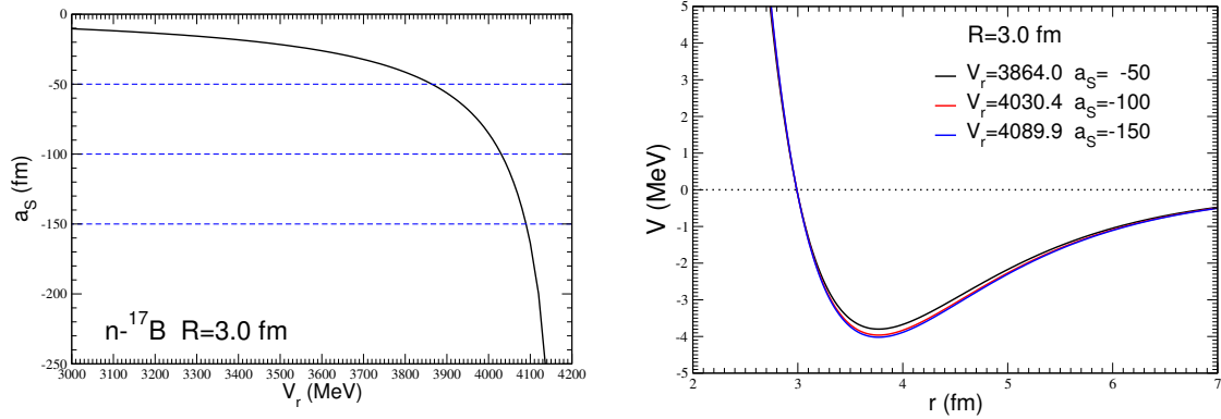
Figure 5: Dependence of the n - ^{17}\text{B} scattering length a_S on V_r for R = 3 fm (left panel). The dashed lines correspond to some selected values of a_S = -50, -100, -150 fm, for which V_{n^{17}\text{B}} have been drawn (right panel).
