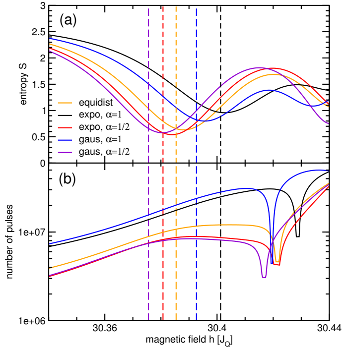
Figure 5: Residual entropies (panel a) and number of pulses (panel b) for a convergence within 1% ( p_{\text{thresh}} = 0.0 ) for N = 3 , J_{\text{max}} = 0.1J_Q , and z = 0.1 for the equidistant parametrization in (8) (legend “equidist”), the exponential parametrization in (9) (legend “expo”) and the Gaussian parametrization in (10) (legend “gaus”). The vertical dashed lines indicate the estimates for the entropy minima which are shifted from the resonances without interactions according to (11).
