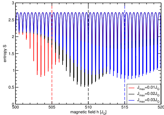
Figure 7: Residual entropy as function of the applied magnetic field for N = 3 , z = 1/1000 and various values of J_{\max} . The shifts indicated by the dashed lines correspond to the estimate (48).
