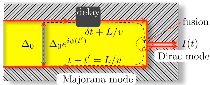
Figure 3: Geometry described by the scattering matrix (7.1).
