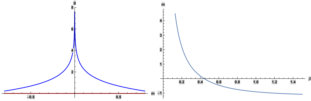
Figure 2: Left: real (blue) and imaginary (red) components of the Fisher information metric (44) for the 1d free fermion theory corresponding to the 2d classical Ising model. Note that the metric obtained via the mapping in [50] is only valid near the critical point m_c = 0 . Right: plot of the mass (46) as a function of \beta = \beta J = \beta K , from which we see that the free fermion mass vanishes precisely at the critical temperature (41), corresponding to the phase transition in the 2d model where one expects to find a conformal field theory. The mass also takes opposite signs on either side of the critical line in fig. 1 that matches the direction of divergence in the 2d curvature, i.e., we find m > 0 on the side nearer the origin and m < 0 on the side nearer \beta J = \beta K \rightarrow \infty .
