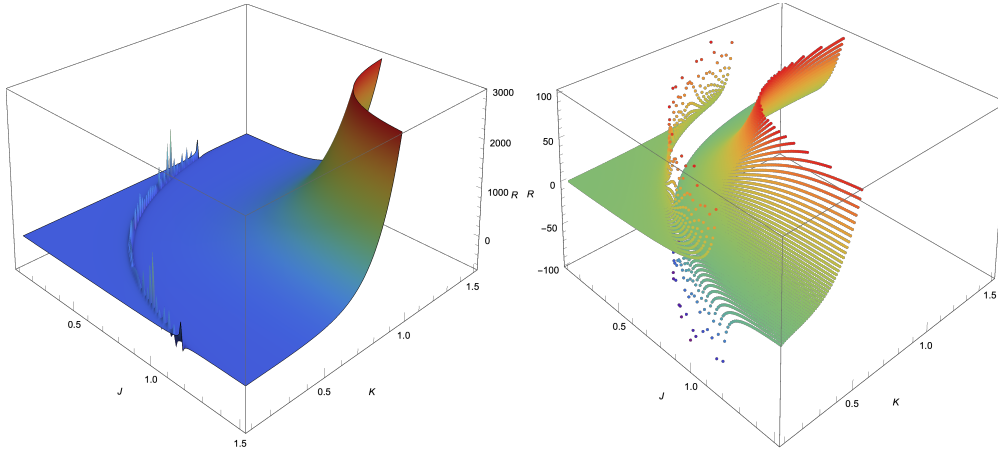
Figure 1: Numerical evaluation of the Ricci scalar (39) for the 2d Ising model, using a uniform grid of 141 \times 141 = 19,881 points between J, K \in \{0.1, 1.5\} (with \beta = 1 ). In the left figure, we have interpolated between points to better show the global features of the curvature: it diverges as J, K \rightarrow \infty , has a discontinuity along the critical line (40) (rendered as the jagged line of spikes by Mathematica’s interpolation attempts), and is otherwise approximately flat. In the right figure, we have plotted the data without interpolating, as well as restricted the vertical range to R \in \{-100, 100\} , to better show the discontinuity along the critical line (40). One sees clearly that the curvature diverges in opposite directions depending on which side one approaches from. We shall see below that this corresponds to the sign of the mass in the corresponding free fermion theory on either side of the phase transition, cf. fig. 2.
