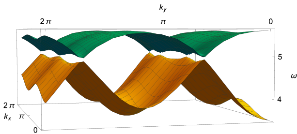
FIG. 6: (Color online.) The two spin wave bands \omega_{\pm} when a strong in-plane field is present. The parameters are chosen J_{zz} = 1 ; J_{\pm} = 0.9 ; J_{\pm\pm} = 1 ; J_{\pm z} = 0.3 ; v = 5 .
