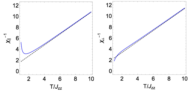
FIG. 2: Susceptibilities versus temperature. The dashed black lines show the Curie-Weiss law, and the solid blue lines plot the inverse of equation (8).
