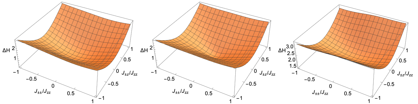
FIG. 3: (Color online.) The dependence of \Delta H (defined in equation (13)) on J_{\pm\pm}/J_{zz} and J_{\pm z}/J_{zz} , with fixed values of J_{\pm}/J_{zz} . Left: J_{\pm}/J_{zz} = 1 , middle: J_{\pm}/J_{zz} = 0.2 , right: J_{\pm}/J_{zz} = -0.5 . In the first two panels, the linewidths are minimal at the “most isotropic” points J_{\pm\pm} = J_{\pm z} = 0 . In the right panel, we depict the case J_{\pm}/J_{zz} < 0 , where the in-plane exchange is ferromagnetic. The linewidths \Delta H in the three plots are in the units \mu_B g(\theta)/\sqrt{2\pi} .
