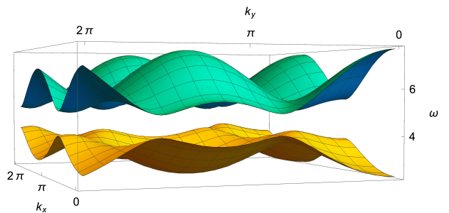
FIG. 4: (Color online.) The two spin wave bands \omega_{\pm} when a strong field in the z -direction is applied. The parameters are chosen as J_{zz} = 1 ; J_{\pm} = 0.9 ; J_{\pm\pm} = 1 ; J_{\pm z} = 0.3 ; u = 5 .
