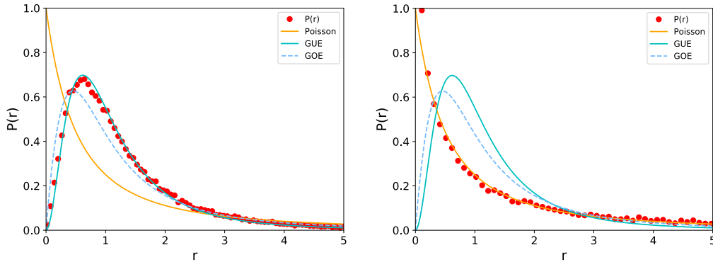
Figure 7: ES statistics of states generated by applying Eq. 7 to random product states. Left: W-D distribution for \theta = \frac{\pi}{8} (inserting T gates); right: Poisson distribution for \theta = \frac{\pi}{4} (inserting S gates). The data are obtained for system size N = 12 with n_T = 12 T or S gate inserted, and averaged over 800 realizations of initial states and random Pauli strings.
