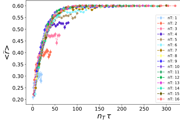
Figure 3: The average \langle \tilde{r} \rangle plotted as a function of n_T \tau past the insertion of T gates, for n_T ranging from 1 to 16, and \tau ranging from 4 to 80 in steps of 4. The system size is fixed to N = 16 . All curves collapse to a universal scaling function \langle \tilde{r} \rangle = h(n_T \times \tau) interpolating between \tilde{r}_{\text{Poisson}} \approx 0.39 and \tilde{r}_{\text{GUE}} \approx 0.6 . The plateau for smaller n_T at large \tau is due to finite-size effect.
