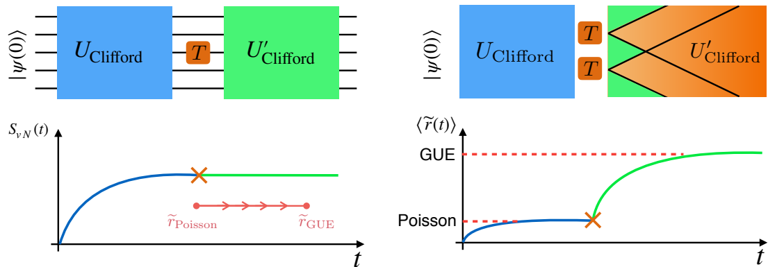
Figure 1: Left: A schematic of the setup considered in this work. Initial product states are first evolved under random Clifford circuits U_{\text{Cl}} until their entanglement entropy reaches maximum. Each circuit is constructed with 500 random non-local Clifford gates to maximize the scrambling speed. A certain number of T gates in one layer are then inserted in the circuit, followed by a second stage of random Clifford evolution U'_{\text{Cl}} also consisting of 500 random non-local Clifford gates. In the thermodynamic limit, the entanglement spectrum approaches a W-D distribution upon inserting a single T gate. Right: A cartoon picture showing the operator spreading of the inserted T gates during the second stage of evolution. Each T gate spreads over a spatial region that grows linearly in time (circuit depth), which sets the timescale for the saturation of the ES statistics to W-D distribution. The onset of W-D statistics occurs when the footprints of the inserted T gates cover all qubits. For this simulation, we choose instead local Clifford gates, so that time is measured in terms of circuit depths.
