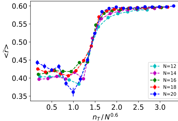
Figure 6: The infinite-time average \langle \tilde{r}(\tau \rightarrow \infty) \rangle versus n_T/N^{0.6} for the special case in which U'_{\text{Cl}} = U_{\text{Cl}}^{-1} , for systems sizes N = 12, 14, 16, 18 and 20 . All curves collapse to a universal scaling function \langle \tilde{r} \rangle = g(n_T/N^{0.6}) interpolating between \tilde{r}_{\text{Poisson}} \approx 0.39 and \tilde{r}_{\text{GUE}} \approx 0.6 . The numbers of realizations are the same as in Fig. 4. When not visible, the error-bars are smaller than the size of the data points.
