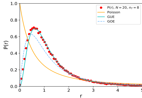
Figure 5: The ES level spacing distribution P(r) for N = 20 with n_T = 8 T gates inserted.
