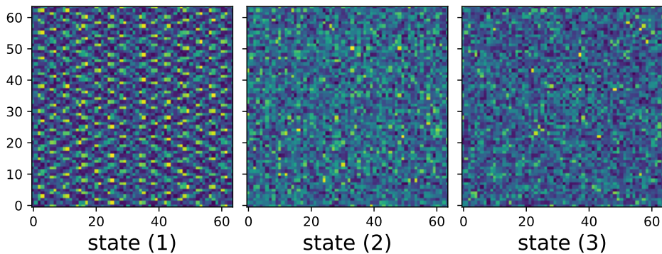
Figure 2: (Color Online) Color map of the matrix |\Psi(x_A, x_B)| under a bipartitioning of the system for (1) a state evolved with a Clifford circuit; (2) a state evolved with the composite quantum circuit in Fig. 1 with n_T = 12 T gates inserted; (3) a random state with entries drawn from a Gaussian distribution. Blue (darker) corresponds to smaller values of |\Psi(x_A, x_B)| and yellow (lighter) corresponds to larger values. The system size is N = 12 .
