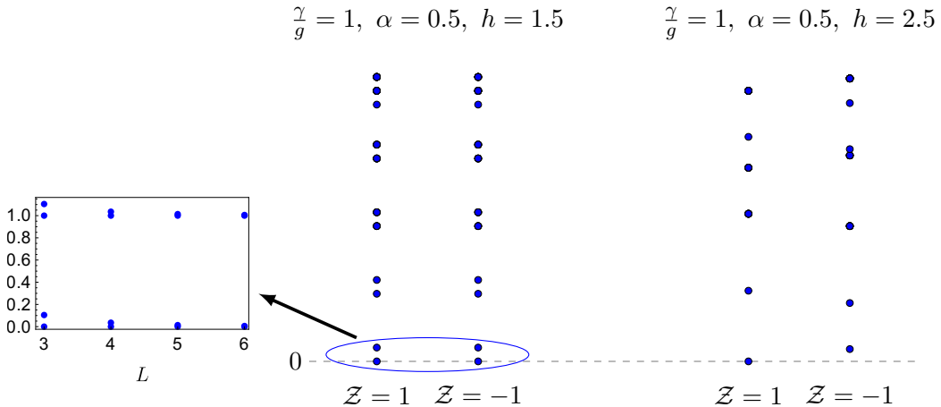
Figure 3: (Negated real part of the) spectrum of the Liouvillian for the topological model with open boundary conditions, split according to the value of the parity \mathcal{Z} = \pm 1 , for values of the parameters inside the topological (left) or topologically trivial (right) phase. In the former case, the inset shows the first two eigenvalues in both sectors for increasing system sizes.
