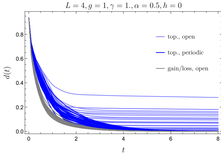
Figure 8: Comparison of the distance to equilibrium for the topological model for open and periodic boundary conditions, as well as the gain/loss model with open boundary conditions, on a system of size L = 4 and starting from randomly drawn initial states (restricted to be pure quantum states at time 0).
