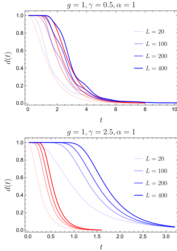
Figure 6: Distance to equilibrium in the topological model for the Ising chain in zero magnetic field ( \alpha = 1, h = 0 ) starting from two different classes of initial states, in the regimes \gamma > 2g , \gamma < 2g and for different sizes L . The blue curves correspond to the least mixed state at all time (“worst choice” initial conditions), while the red curves correspond to a product of single-sector commuting matrices, which for \gamma > 2g seems to be the fastest-mixing state.
