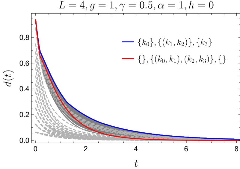
Figure 4: Evolution of the distance to equilibrium in the gain/loss model for L = 4 . The dashed light gray lines correspond to randomly drawn initial density matrices with various levels of mixing, while the darker gray lines correspond to initial pure quantum states. The colored lines are analytical predictions for initial density matrices of the type (46). We recall the notation k_j = \frac{2\pi j}{L} for the momenta, but emphasize that in the present case the results are insensitive to any permutation of the latter.
