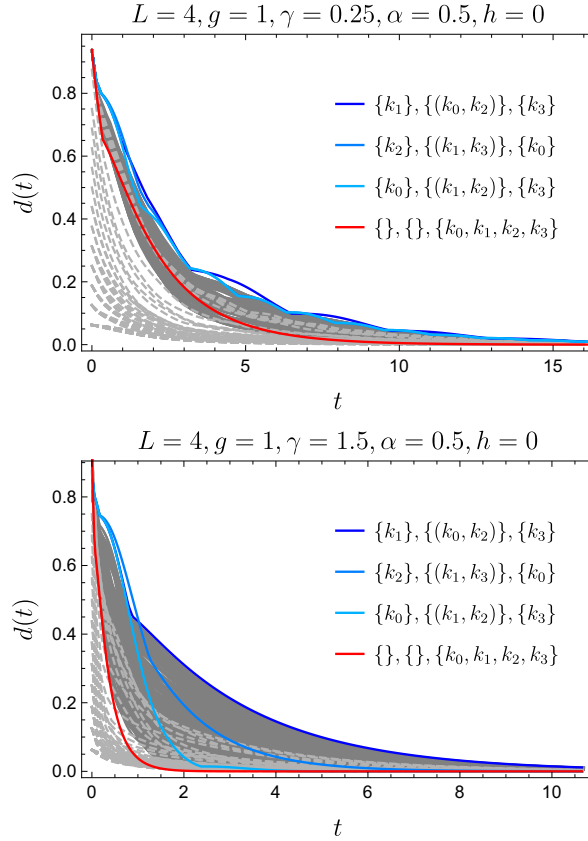
Figure 5: Evolution of the distance to equilibrium in the topological model for L = 4 and various choices of parameters. The dashed light gray lines correspond to random initial density matrices with various levels of mixing, while the darker gray lines correspond to initial pure quantum states. The colored lines are analytical predictions for initial density matrices of the type (46), where we recall the notation k_j = \frac{2\pi j}{L} .
