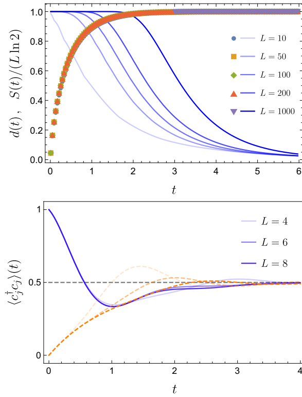
Figure 7: (Left) Evolution of the distance to equilibrium (blue curves) and the von Neumann entropy (colored dots) of the slowest-mixing state for various system sizes in the gain-loss model with \gamma = 0.5 . (Right) Evolution of the fermion occupation number at site L (blue curves) and in the middle of the chain (orange curves) for the gain/loss model with \alpha = 0 , h = 0 , \gamma = 0.5 , starting from the state with one particle at site L and zero elsewhere.
