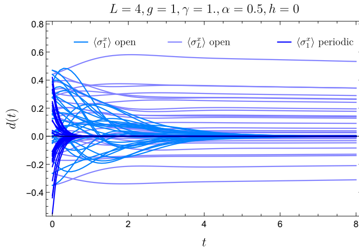
Figure 9: Evolution of the “local” observables \langle \sigma_1^x \rangle and \langle \sigma_L^x \rangle for the topological model with open and periodic boundary conditions, starting from randomly drawn initial states (restricted to be pure quantum states at time 0).
