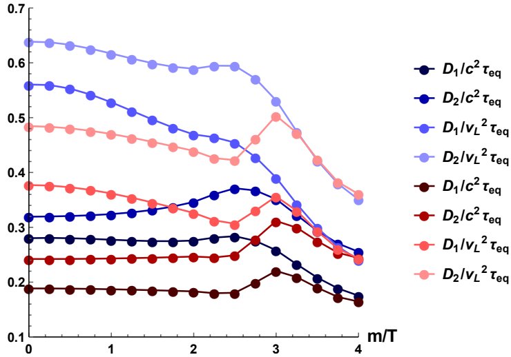
Figure 8: A verification of the universal upper bound (49) imposed by causality. The blue points are for \mu/T = 3 while the red for \mu/T = 5 .
