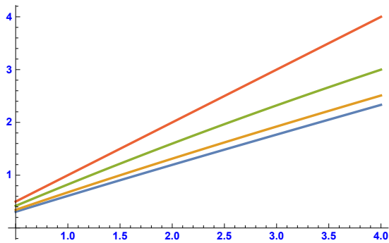
FIG. 2: The plot of \ln[3\pi G_n(\mathbf{k})(1 + A(g_n^{*'})^2)] against \ln[1/|\mathbf{k}|] , where G_n(\mathbf{k}) is given by Eq. 20. From top to bottom, A(g_n^{*'})^2 = 0, 1/2, 2, and 5 .
