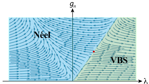
FIG. 1: The coupled RG flow of \lambda and g_n based on Eq. 11. A new fixed point (\lambda^*, g_n^*) = (\frac{2\epsilon_n}{\pi}, \frac{4\epsilon_n}{\pi}) is found, which separates two phases: the phase where \lambda \rightarrow +\infty is the VBS phase, and the phase with (\lambda, g_n) \rightarrow (-\infty, +\infty) is the long range Néel order at the 1d boundary. But on the Néel order side of the phase diagram, the RG flow is complicated and nonmonotonic, hence it may take a long RG scale, or a large system size to finally reveal the true long range order.
