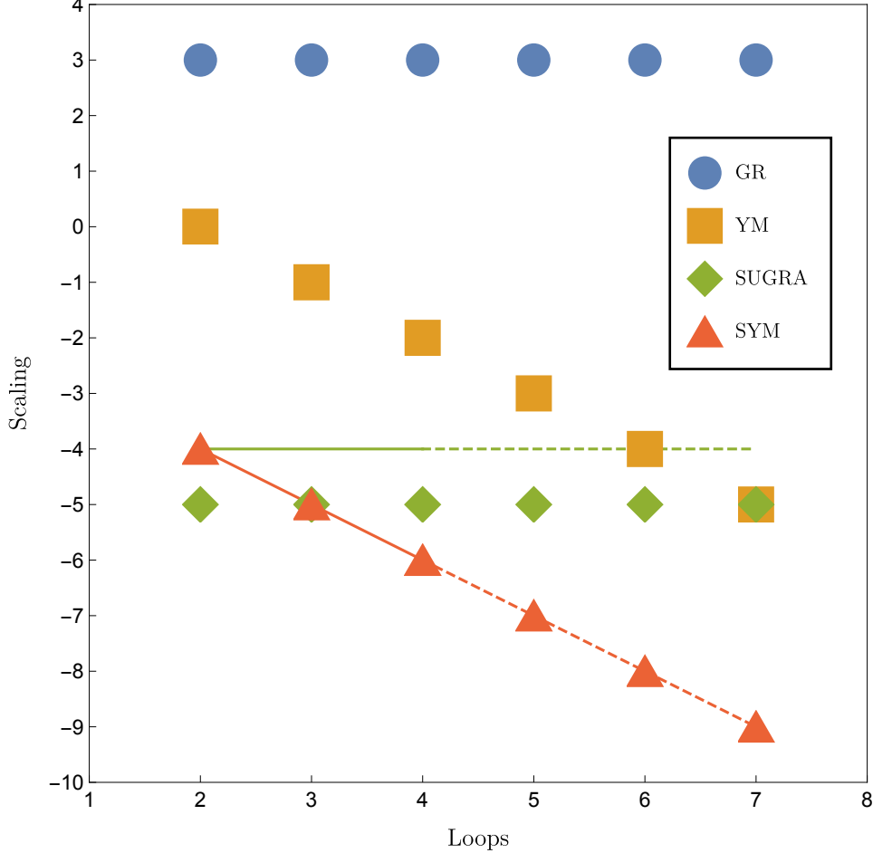
Figure 2: UV scaling of \mathcal{N} = 8 SUGRA, (planar) \mathcal{N} = 4 SYM, pure GR, and pure (planar)YM multi-particle unitarity cuts under four-dimensional deformations with results up to seven loops. The Scaling axis labels the leading t behavior of the cuts as t \rightarrow \infty . The thin lines denote the scaling in D -dimensions, where the continuous part has been checked explicitly and the dashed part is conjectured. There is an overall improvement of one power in the large t limit of gravity cuts with respect to D -dimensions; the same is not true for Yang-Mills.
