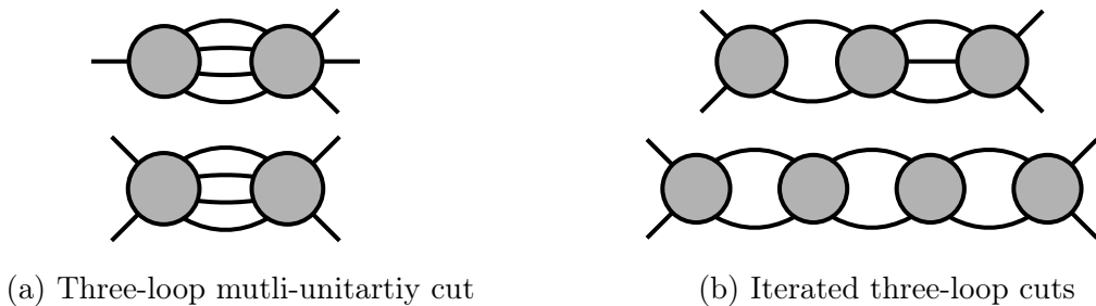
Figure 4: Cut topologies considered in the UV construction of the three-loop four-point amplitude in \mathcal{N} = 8 SUGRA.
