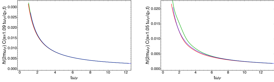
Figure 9: Correlation function C(x, t) \equiv \langle \sigma(x, t) \sigma(0, 0) \rangle in a thermal state for x = 2\alpha t as a function of t at c = 4 , for \beta = 1 and D = 0.38 (left) and \beta = 3 and D = 0.386 (right). The three curves depict the real part (red), the modulus (green) and the GHD approximation (dashed blue).
