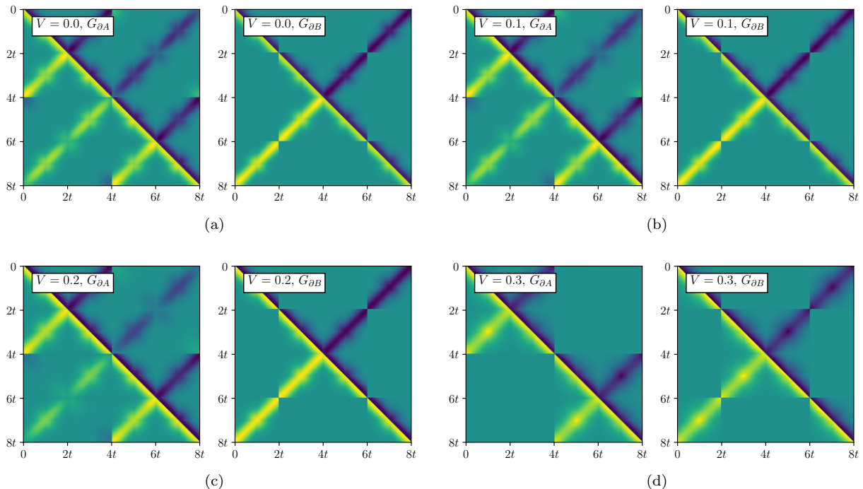
Figure 6. Green's function profile on the subsystem boundary \partial A and \partial B for various V at t = 8 . Initial condition Type 2(QA) is applied. As V increases, the saddle point solution gradually changes from a replica quasi-diagonal solution to a replica diagonal solution.
