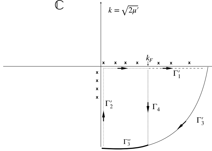
Figure 3: Contour integrals used in the integral representations of the kernel in terms of the variable k = \sqrt{2m\mu'}/\hbar . Crosses indicate the poles of the Green's function in the complex plane of k . The contours \Gamma'_i for i = 1, 2, 3 correspond to the contours \Gamma_i shown in Fig. 2 when mapped into the k plane. Note that the contour \Gamma'_2 has two components: one vertical, and one horizontal going from k = 0 to k = k_F . The contour \Gamma''_3 denotes a portion on \Gamma'_3 , shown in bold, which is useful for later purpose. The contour \Gamma_4 = (k_F, k_F - i\infty) , which is useful for asymptotic analysis, is also shown.
