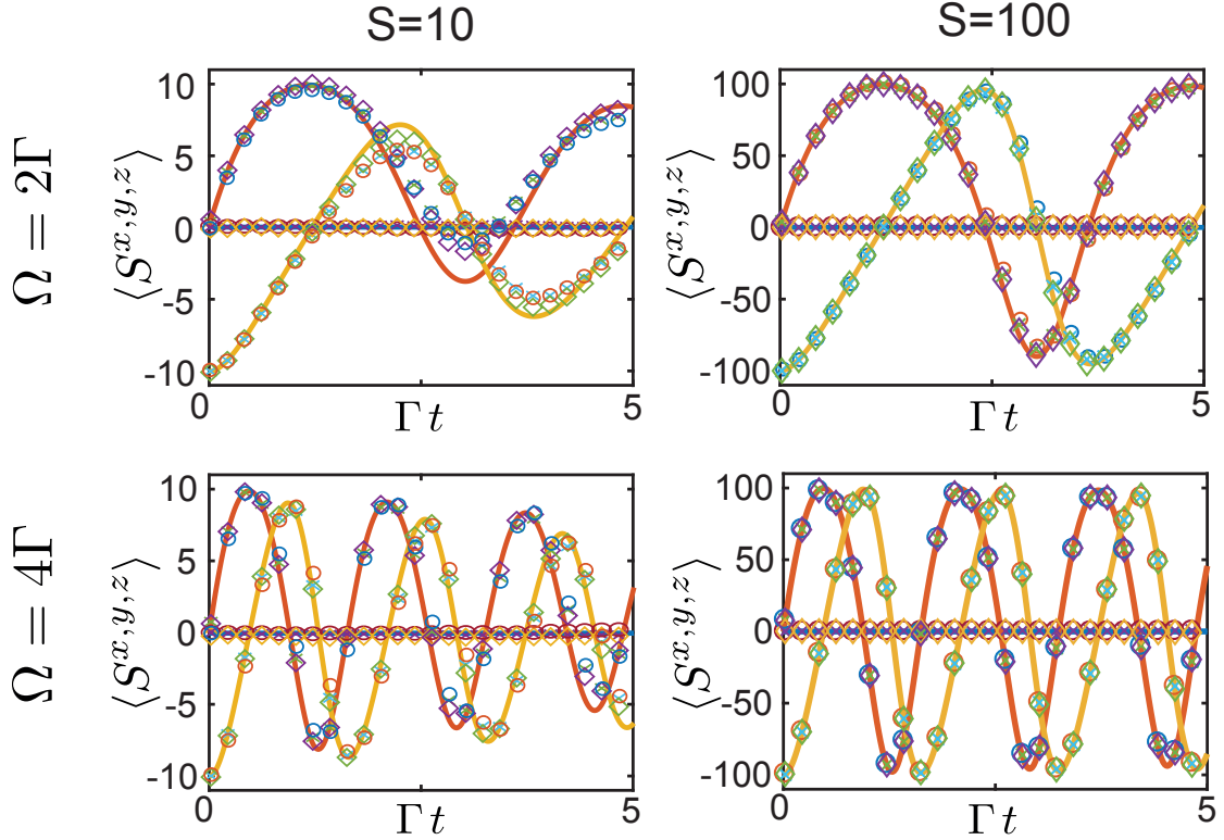
Figure 3: Time evolution of a driven collective spin in the presence of dissipation, as described by Eq. (29). The solid lines represent the exact dynamics of the spin expectation values \langle S^z \rangle (yellow line), \langle S^y \rangle (red line) and \langle S^x \rangle (blue line), while the crosses, diamonds and circles are obtained from the stochastic sampling of the P -, the Q - and the Wigner-distribution, respectively. For this simulation, the system is initialized in the fully polarized state |S^z = -S\rangle .
