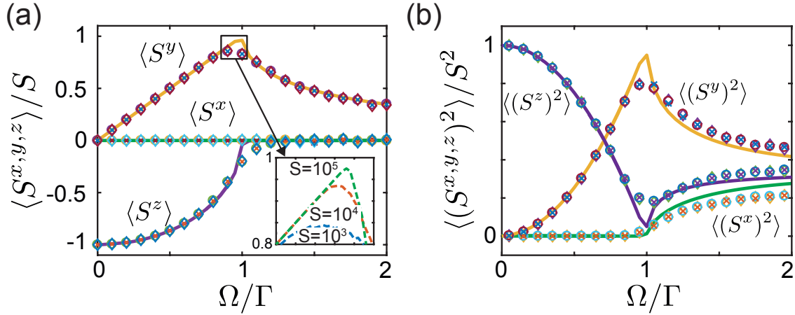
Figure 4: Simulation of the steady state of a driven spin system described by Eq. (29). The two plots show (a) the mean values and (b) the fluctuations of the three components of a spin with S = 1000 . The solid lines are obtained from the exact solution for the steady state of this system [17, 35, 36], while the crosses, diamonds and circles are obtained from a stochastic sampling of the P -, the Q - and the Wigner-distribution. The inset in (a) shows the simulations of the Wigner distribution for even larger spin numbers S around the transition point \Omega / \Gamma = 1 . The steady state was obtained by time averaging after t = 40\Gamma^{-1} for another period of \Delta t = 10\Gamma^{-1} and for n_{\text{traj}} = 2500 .
