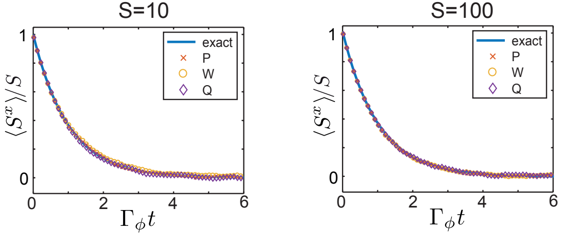
Figure 2: Dephasing of a collective spin as described by Eq. (24). For this plot, it is assumed that the system is initially prepared in a spin coherent state pointing along the x -direction, |S^x = S\rangle , and the successive evolution of \langle S^x \rangle(t) is shown as a function of time. For this example the other two spin components vanish up to statistical errors. The exact results obtained from the full master equation are compared with stochastic simulations of Eq. (27) and Eq. (28) for k = 0, \pm 1 . To obtain this data n_{\text{traj}} = 1000 trajectories were simulated.
